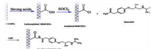
Scheme1: Strategy for modified functionalized multiwall carbon nanotubes (FMWCNT) synthesis [15].
