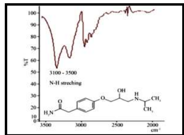
Fig:5: Pure atenolol FTIR spectrum [16].
