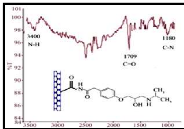
Fig: 6: Modified functionalized multiwall carbon nanotubes (FMCNT) FTIR spectrum [17].
