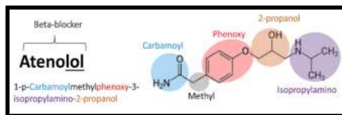
Fig:1: The molecular and structural formula of atenolol [2].
