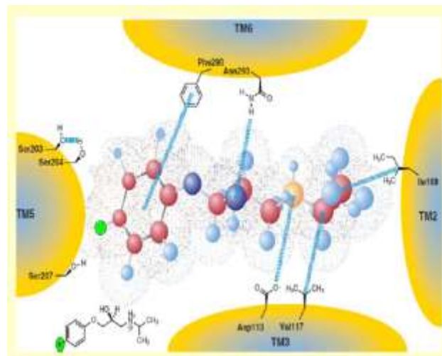
Fig:3: Interactions of atenolol functional groups with the receptor [10].
