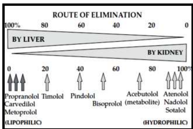
Fig:2: Schematic chart of elimination routes [2].
