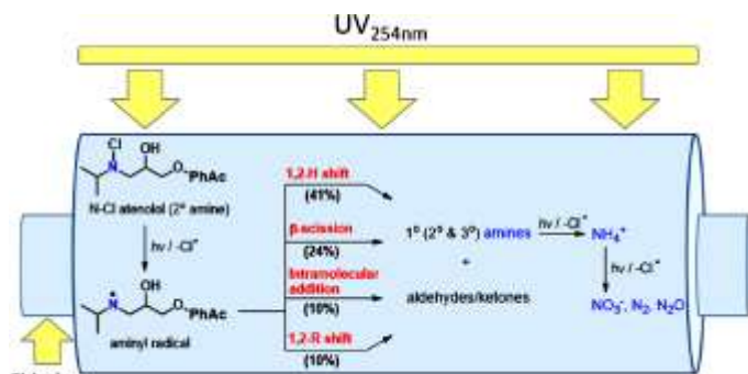
Fig: 4: Transformation of atenolol (ATN) [14].
