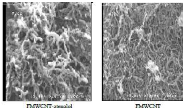
Fig:7: SEM images of functionalized multiwall carbon nanotubes (FMWCNT) and FMWCNT-atenolol [17].
