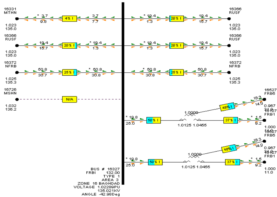
Figure (2) Farabe-132kV bus and connections load flow results, one DG ad
