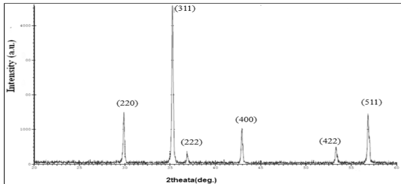
Figure (4) XRD patterns of sintered at 1373 0 k sample (E2) Ni_{0.6}Zn_{0.3}Mg_{0.1}Fe_2O_4 .
