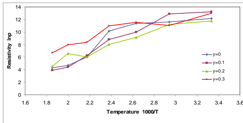
Figure (7) Represents resistivity as a function of temperature (1/T) of MgNiZn ferrites with different composition
