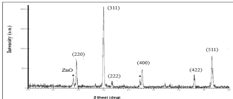
Figure (5) XRD patterns of sintered at 1373 0 k sample (G2) Ni_{0.4}Zn_{0.3}Mg_{0.3}Fe_2O_4 .
