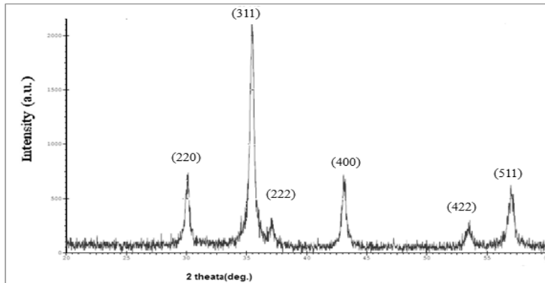
Figure (3) XRD patterns of calcined at 773 0 k sample (G) Ni_{0.4}Zn_{0.3}Mg_{0.3}Fe_2O_4 .
