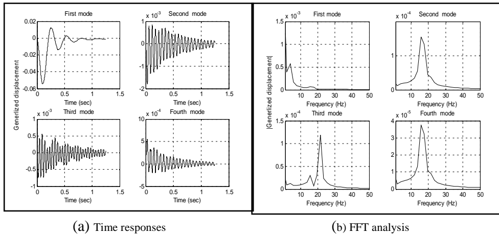
Figure (6) Theoretical responses of the generalized displacements and their FFT analysis for plate type-B at V=15 (m/sec) (below flutter speed)
