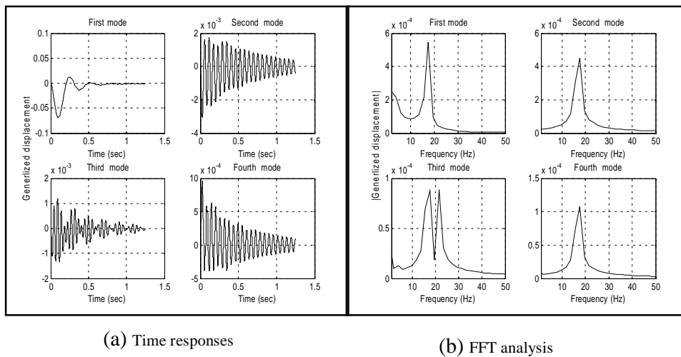
Figure (7) Theoretical responses of the generalized displacements and their FFT analysis for plate-B at V=20 (m/sec) (below flutter speed)
