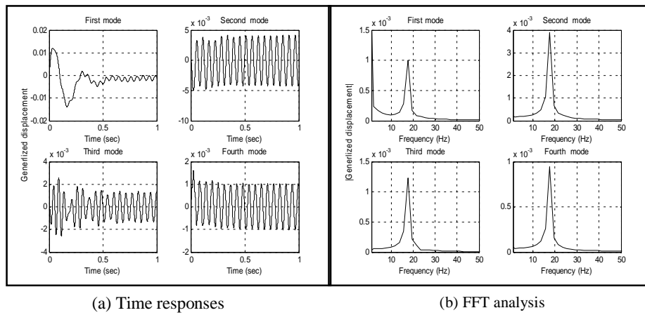
Figure (8) Theoretical responses of the generalized displacements and their FFT analysis for plate-B at V=24.7 (m/sec) (flutter condition )
