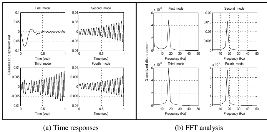
Figure (9) Theoretical responses of the generalized displacements and their FFT analysis for plate-B at V=26 (m/sec)(beyond flutter speed)
