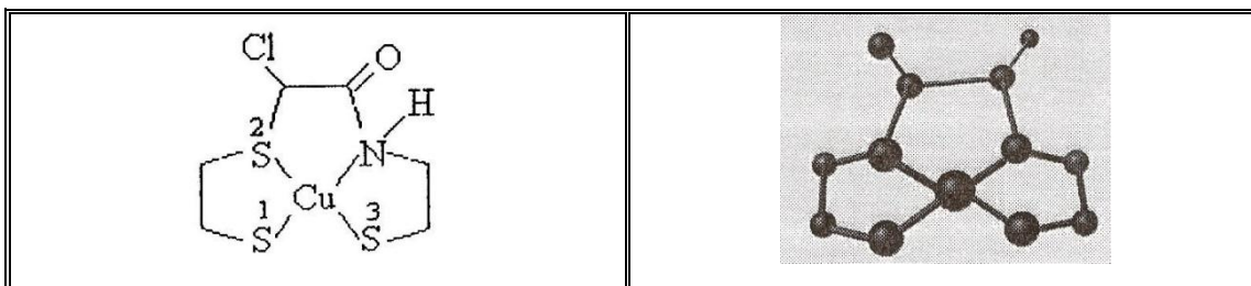
Figure (5) The Proposed Structure for [Cu(HL)]
