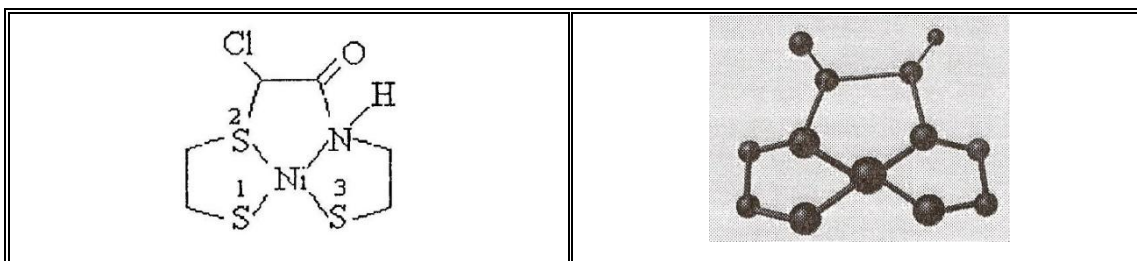
Figure (4) The Proposed Structure for [Ni(HL)]
