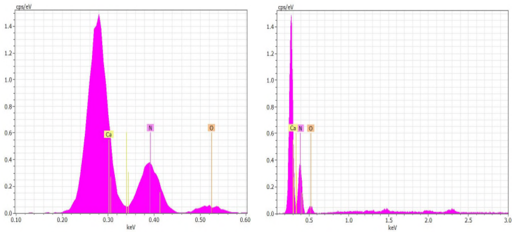
Figure (2): EDS of hydroxyapatite prepared using chemical method.
