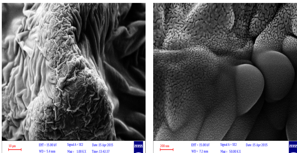
Figure (1): FESEM of hydroxyapatite prepared using chemical method.
