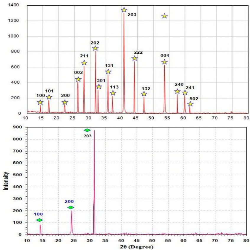
Figure (3): XRD of hydroxyapatite prepared using chemical method.
