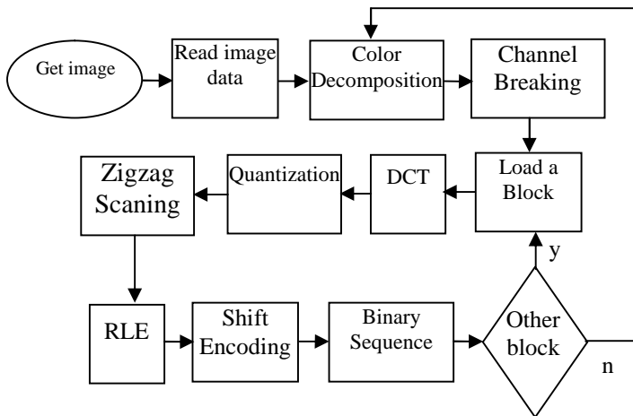
Figure(1) stages of compression.
