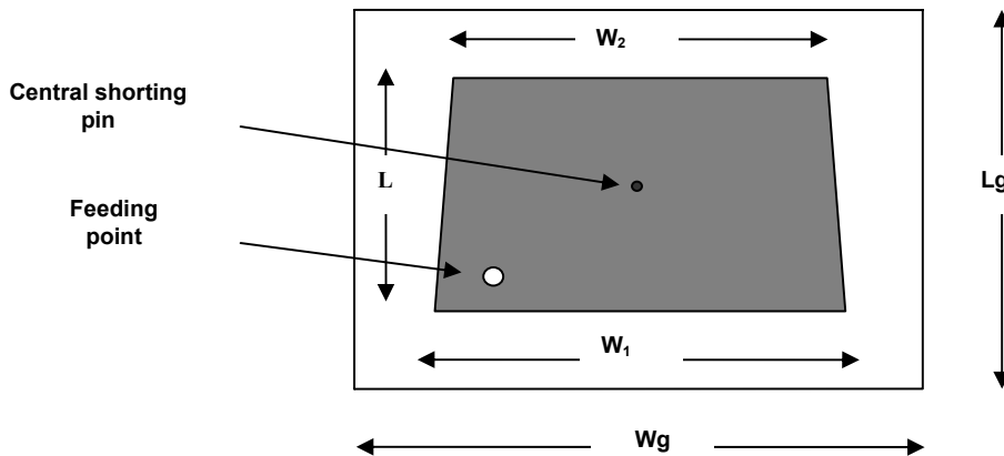
Compact design modified shape that gives broader bandwidth feeding point for both cases with and without central shorting pin and for substrate materials Duroid 5880 and Quartz.
