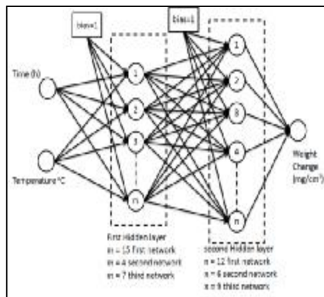
Figure (1) the neural network model.
