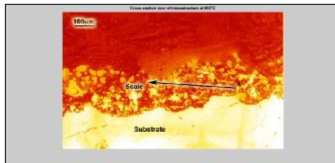
Figure (4) LOM of low alloy steel type-T21 coated with germanium-Doped aluminizing-siliconizing after cyclic oxidation under air at 600oC. (Cross section view).
