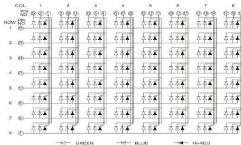
Figure (3) 8x8 Dot Led Matrix.
