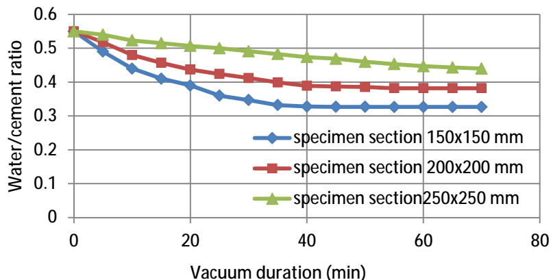
Figure (4) Relation between water/cement ratio and vacuum duration
