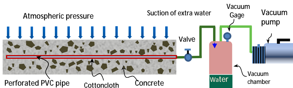
Figure (2) New vacuum dewatering technique
