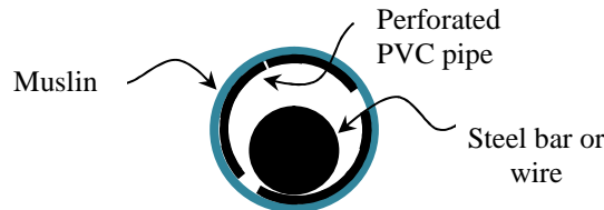
Figure (1) Cross-section of perforated dewatering pipe
