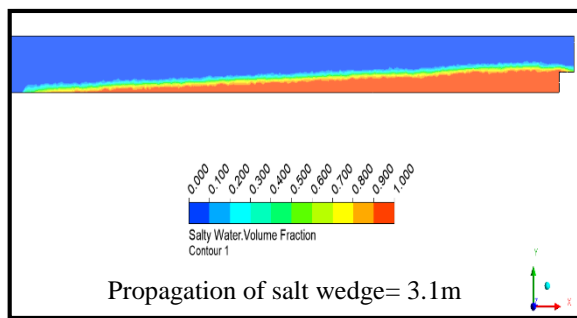
a- Discharge= 45.3 l/min.
