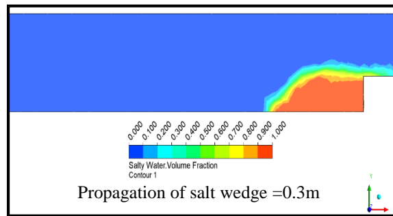
c- Discharge= 78.4 l/min
