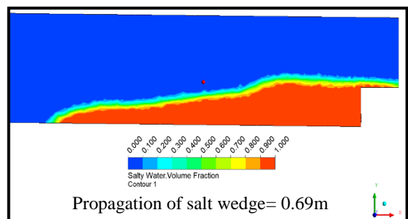
b- Discharge= 61.3 l/min
