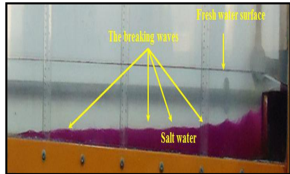
b- laboratory model, (Al-Fuady and Azzubaidi, 2021).
