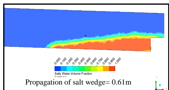
Figure 8. Propagation of salt wedge at different discharges and a slope of 2%.
