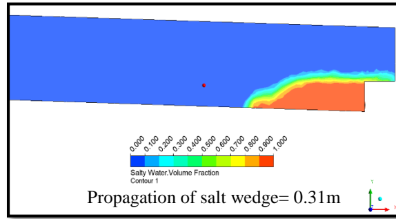
Figure 9. Propagation of salt wedge at different discharges and a slope of 3%.
