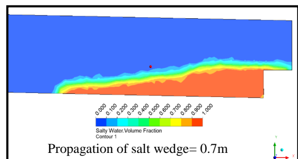
Figure 7. Propagation of salt wedge at different discharges and a slope of 1%..
