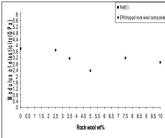
Fig.(9) Modulus of elasticity (E) verse rock wool wt% of EP/chopped rock wool composites.
