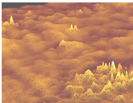
Fig.(8) Defects (voids) inside EP/chopped rock wool composites (sample H).
