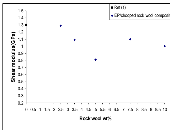
Fig.(7) Shear modulus (G) versus rock wool wt% of EP/chopped rock wool composites.
