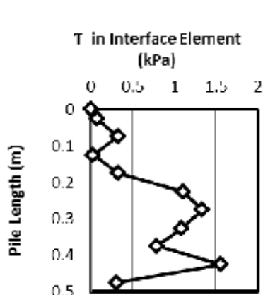
Figure (14) Shear stresses at soil-pile interface for pile with D=2 cm, L=0.5 m.
