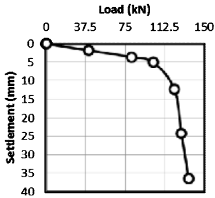
Figure (9) Load-Settlement relation of pile with D= 30 cm and L= 450 cm.
