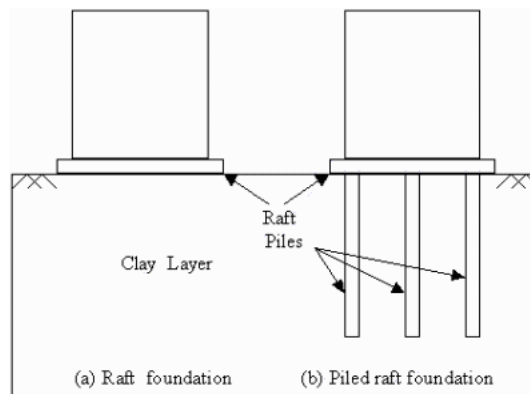
Figure (1) Piled raft foundation [1].
