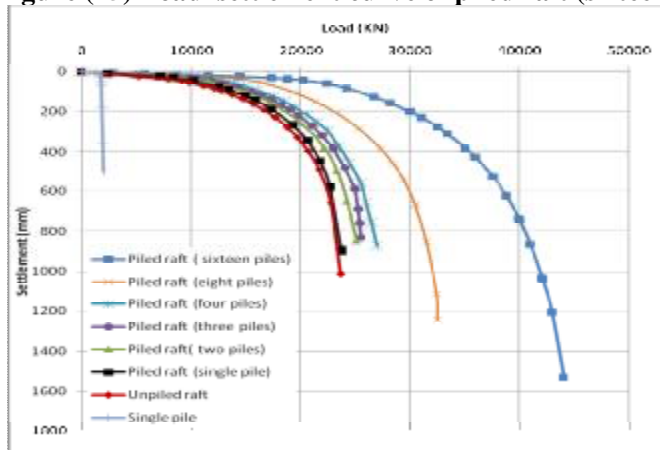
Figure (16) Load–settlement curve for all cases.
