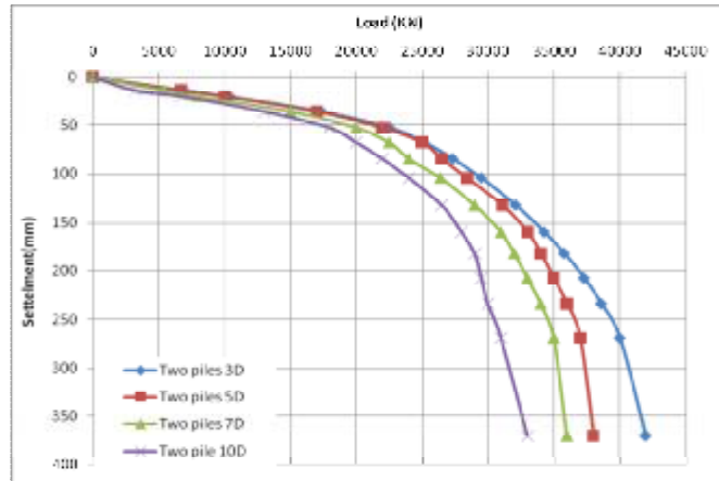
Figure (17) Effect of spacing between piles.
