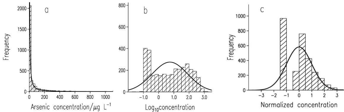
Figure. 2 The concentration of arsenic -Bangladesh (a) no transformation (b) lognormal transformation (c) Hermite polynomial transformation, Gaus et al., 2003 .
