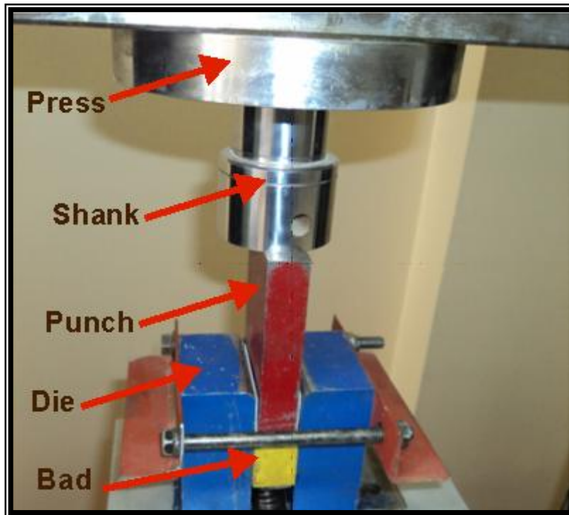
Figure (2) The U-bending die.
