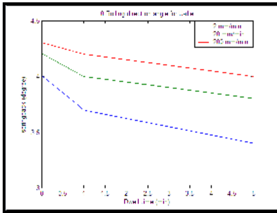
Figure (9) Relationship between dwell time with springback (0°) (45°) dwell
