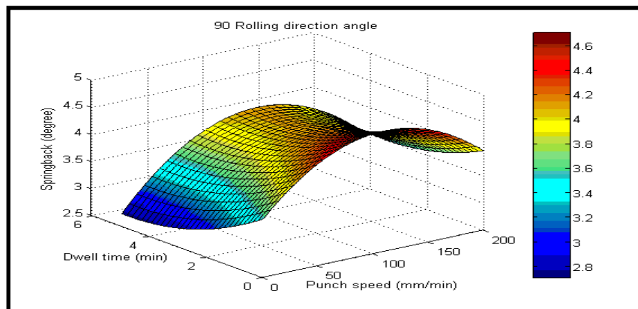
Figure (12) Relationship between the punch speed and dwell time with spring back in 90° direction angle rolling.
