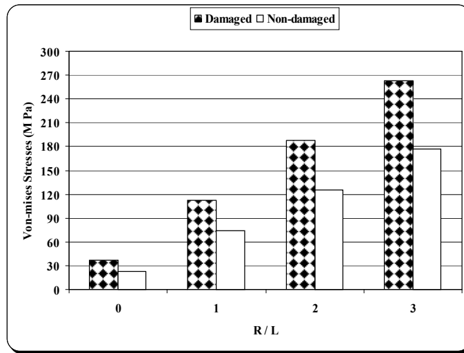
Fig.14. Variation of Von-Mises Stresses With (R/L) (2 nd Model, \Omega=1 , L/W=1 , \alpha = 0 , \theta = 0 ).
