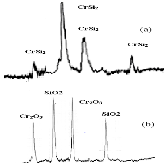
Figure 3. XRD-Phases of low alloy steel coated with Ge-doped Cr-Si .(a) after coating, (b) after oxidation in air at 800 °C.
