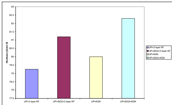
Figure 4: The hardness for composite and hybrid composite before and after SiO 2 addition
