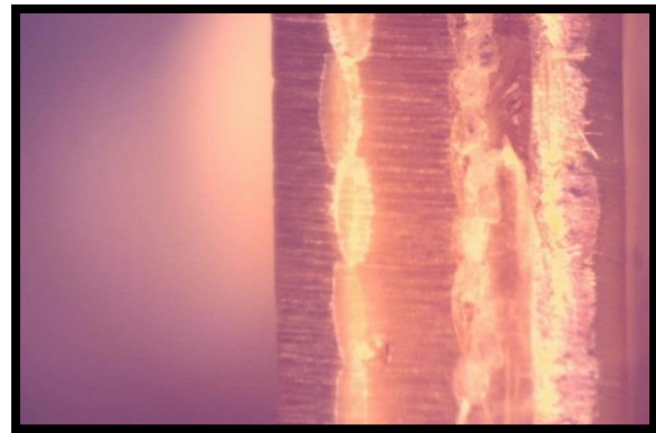
Figure 6: Optical micrograph of composite reinforced with the sequence of layers (Kevlar-Glass-Kevlar)
