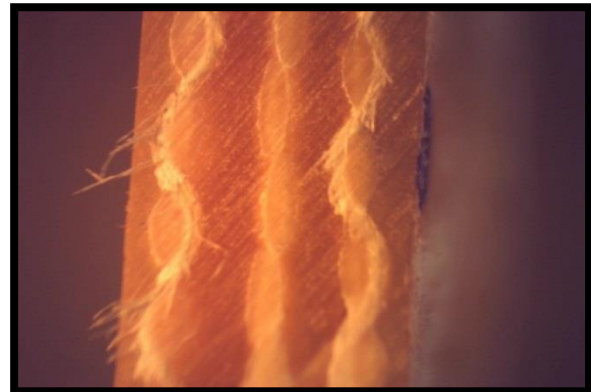
Figure 7: Optical micrograph of the cross section for composite reinforced with three layers of Kevlar fibers and SiO 2 powder
