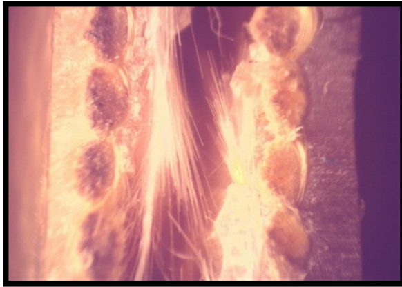
Figure 10: Optical micrograph of the cross sectional fracture surface after flexural test for composite reinforced with the sequence of layers (Kevlar-Glass-Kevlar) and silica powder
