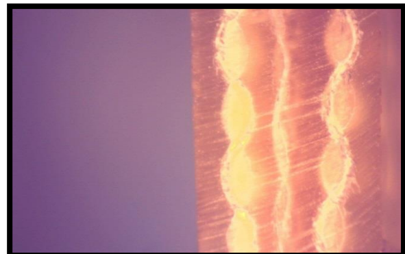
Figure 8: Optical micrograph of the cross section for composite reinforced with the sequence of layers (Kevlar-Glass-Kevlar) and SiO 2 powder
