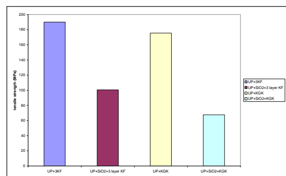
Figure 1: Tensile strength for composite and hybrid composite before and after \text{SiO}_2 addition
