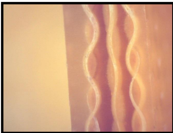
Figure 5: Optical micrograph of the cross section for composite reinforced with three layers of Kevlar fibers
