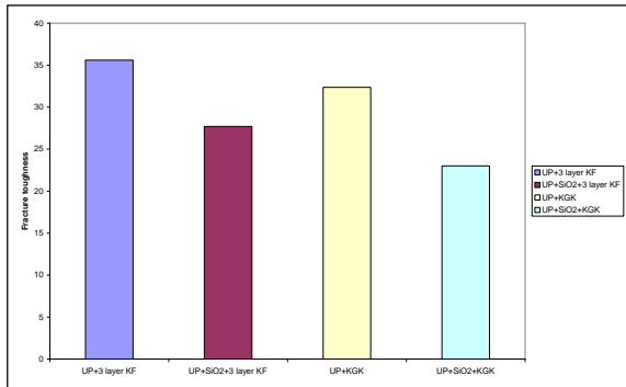
Figure 3: The fracture toughness for composite, and hybrid composite before and after SiO 2 addition
