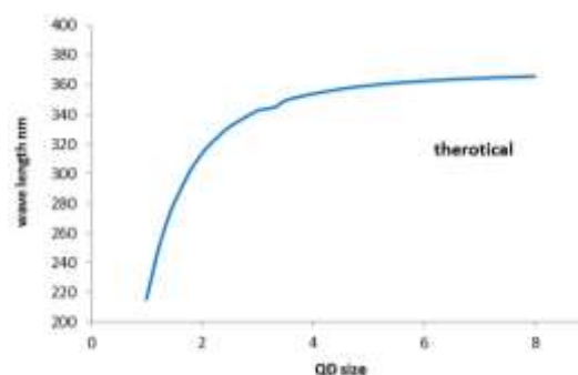
Fig. 6: The wave length variation with quantum dot size of ZnO
