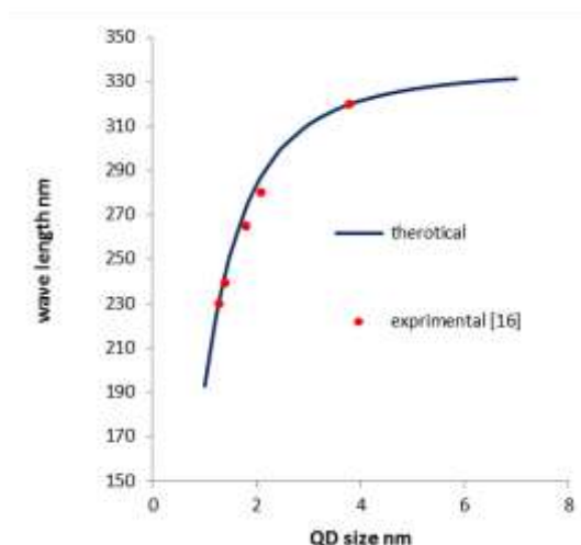
Fig. 5: The wave length variation with quantum dot size of ZnS
