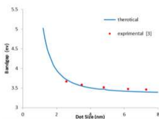
Fig. 3: The variation the bandgap and Dot Size (nm) for ZnO.
