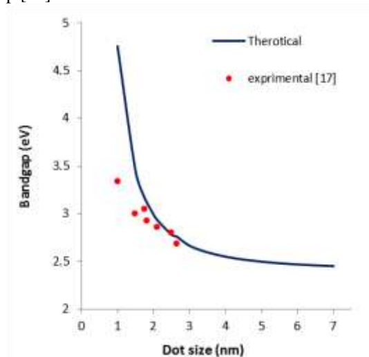
Fig. 1: The variation the bandgap and Dot Size (nm) for CdS
