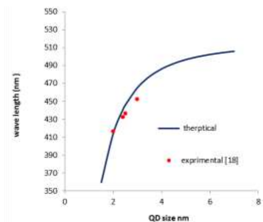
Fig. 4: The wave length variation with quantum dot size of CdS
