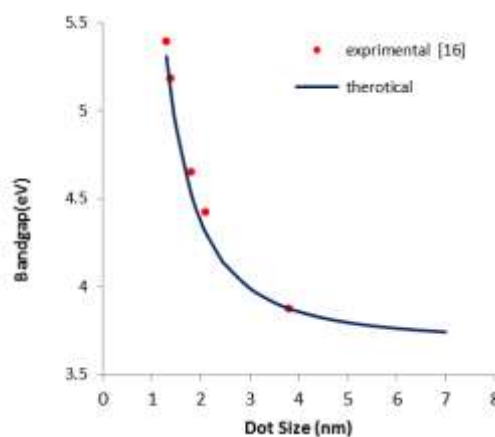
Fig. 2: The variation the bandgap and Dot Size (nm) for ZnS
