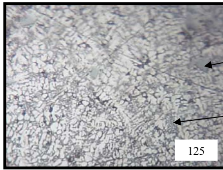
Figure (16) microstructure of Al-12%Si-0.3%NaCl, at pouring temp. 800 °C
