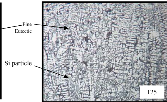
Figure (13) microstructure of Al-12%Si-0.5%NaCl, at pouring temp. 1000 °C
