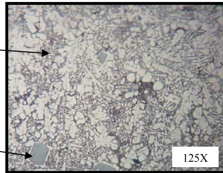
Figure (15) microstructure of Al-12%Si-0.1%NaCl, at pouring temp. 800 °C
