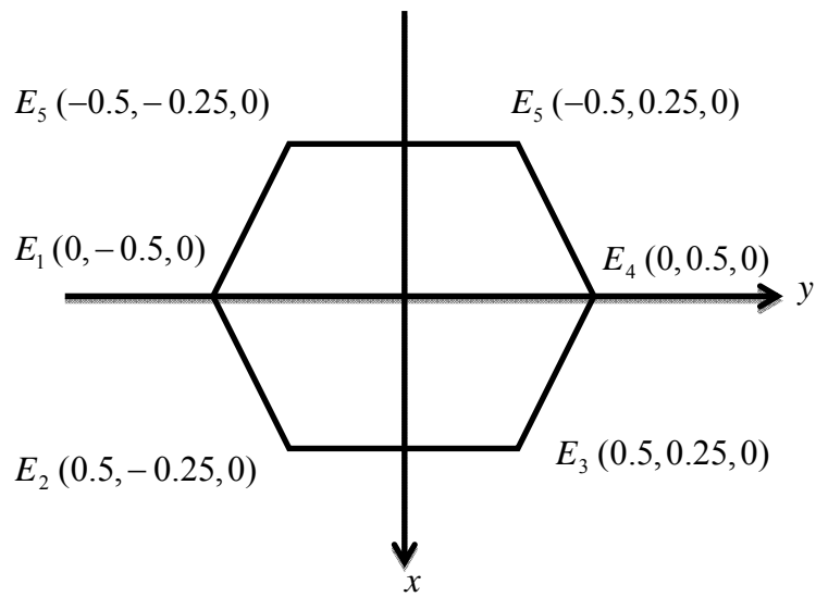
Figure (7): Dimensions of the moving platform with respect to local coordinate system
