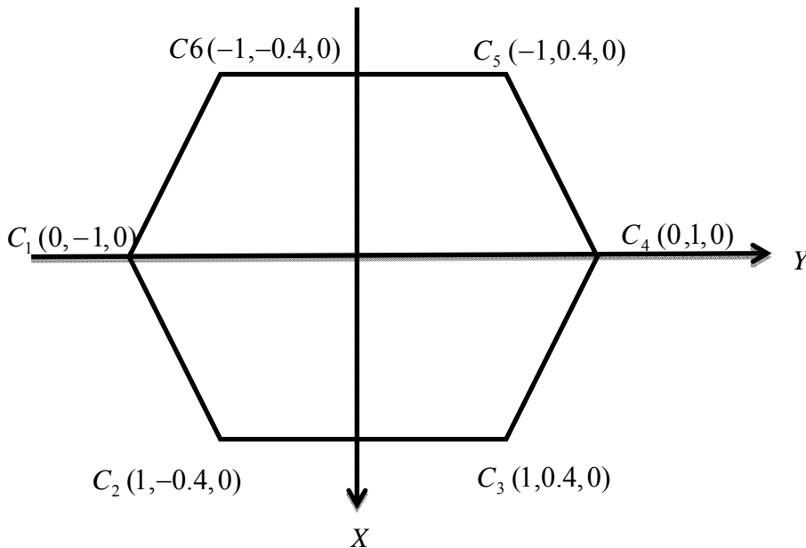
Figure (6): Dimensions of the fixed platform with respect to global coordinate system
