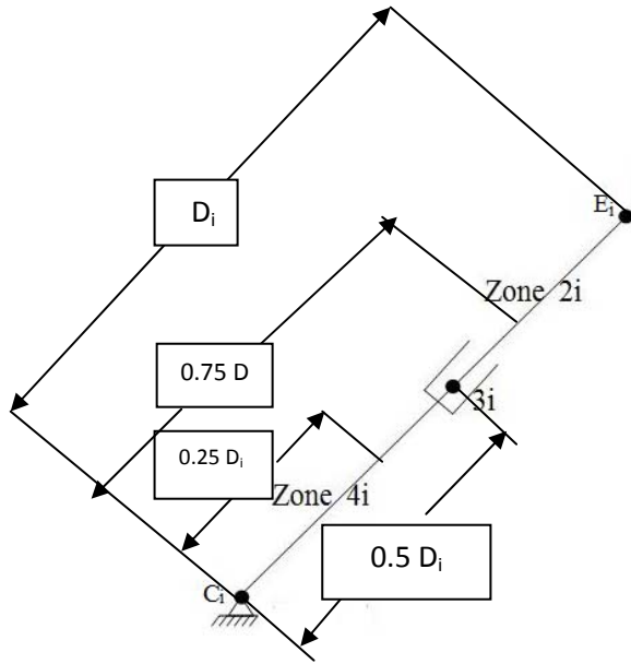
Figure (3) Linkage (i) mechanism
