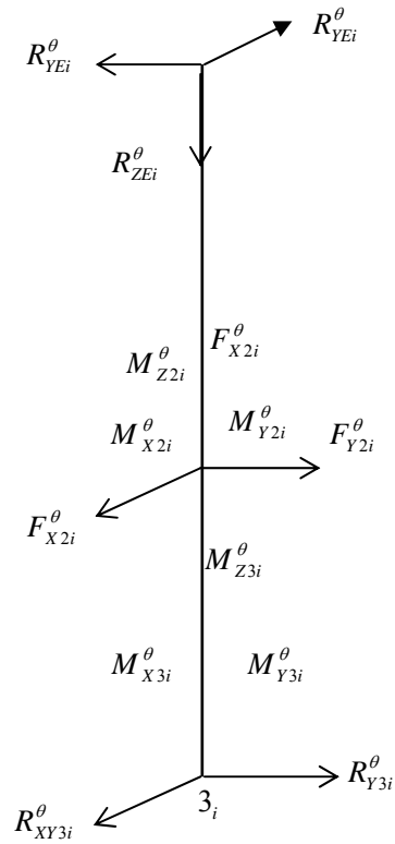
Figure (5) Upper part of the linkage (i)
