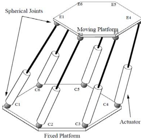
Figure (1) Gough-Stewart mechanism
