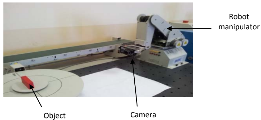
Figure (1) eye on hand robot system configuration
