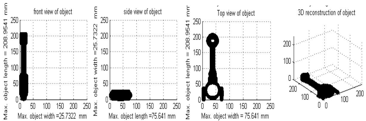
Figure (18) Connected Rod Views and 3D Model
