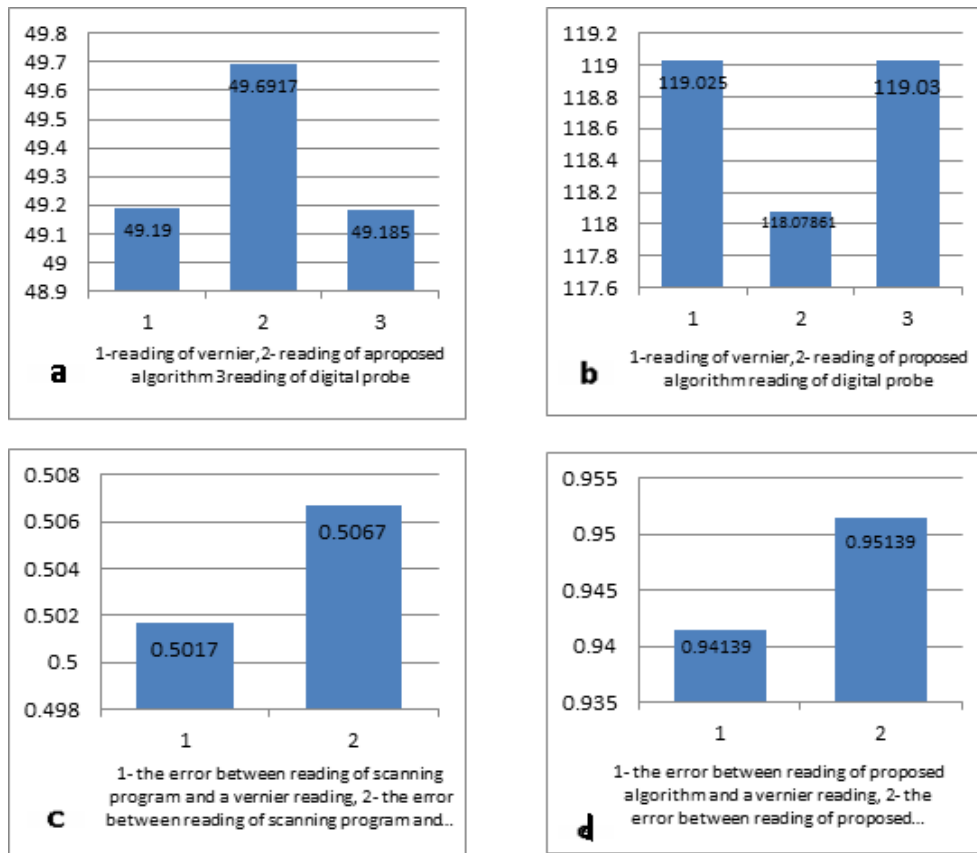
Figure (12) (a,b) comparison of digital vernier, scanning program and digital probe reading, (c,d) comparison the error of dimension for bottle shape.
