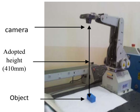
Figure(6) capturing top view picture
