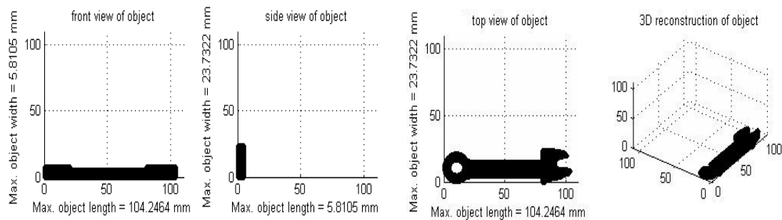
Figure (14) Span Views and 3D Model.
