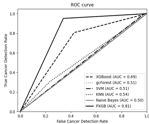
Figure 4: The ROC curves and their AUC values for the GSE68465 dataset
