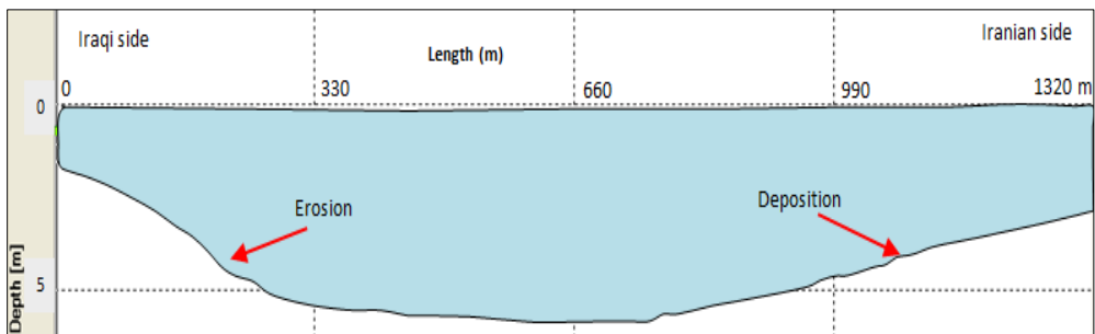
Figure 4. A Cross section of Shatt Al-Arab River in the estuary part.
