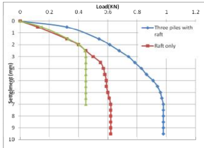
Figure (17) Load–displacement curve for three piles with raft, three piles unraft and raft only of the small model.
