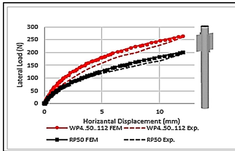
Figure 4: Lateral load versus horizontal displacement for a single winged pile model with a relative the density of 35%
