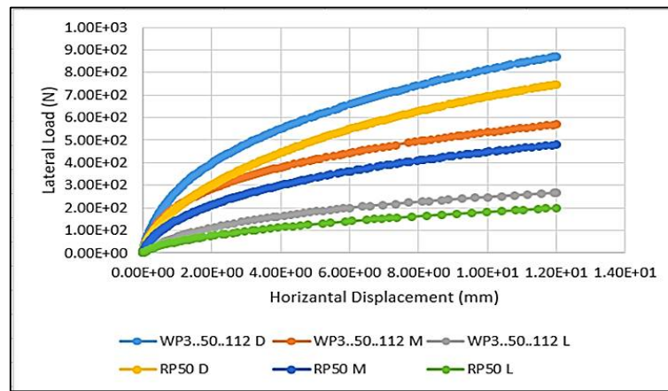
Figure 11: load-displacement curve in various Relative densities ( D_r=35, 60 and 75\% )
