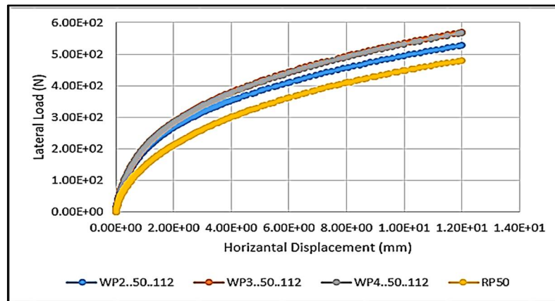
Figure 9: The curves of load-displacement for different Wing Numbers at L/D= 10 and medium relative density
