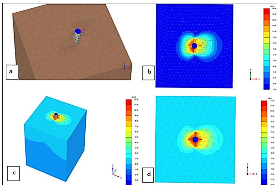
Figure 8: Pile- soil deformation (a and b) total lateral displacement (c and d) lateral displacement for x-direction only
