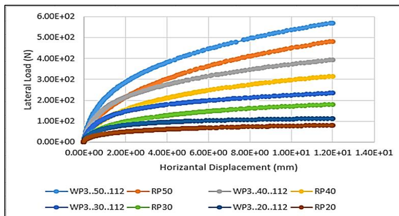
Figure 10: Load-displacement curves for different slenderness's ratios (10, 8, 6, 4) at a medium relative density
