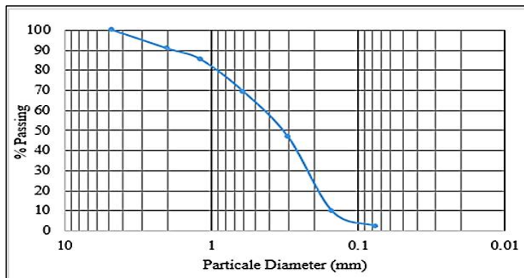
Figure 2: The grain size distribution
