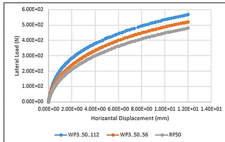
Figure 5: The load-displacement curve at different wing lengths for L/D=10 and Medium sand
