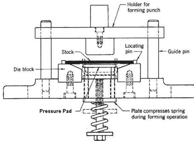
Figure (7) U-Die
