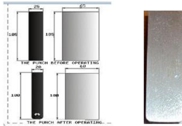
Figure (9) Punching of U-die processes (a) drawings (b) photo
