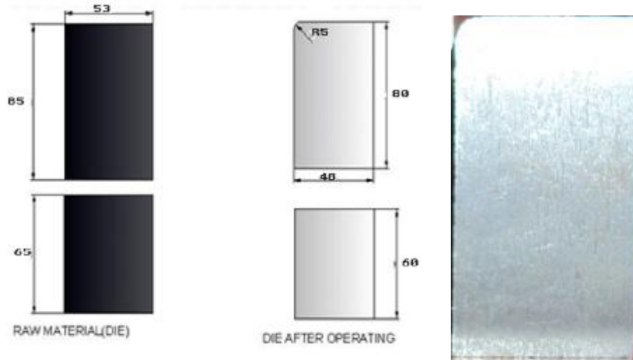
Figure (9) Punching of U-die processes (a) drawings (b) photo
