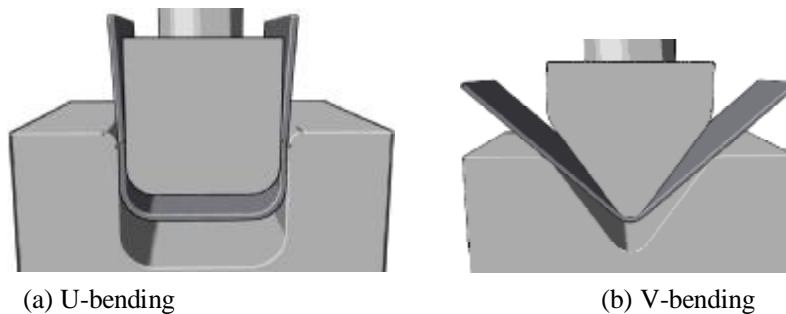
Figure (1) V-die and U-die processes
