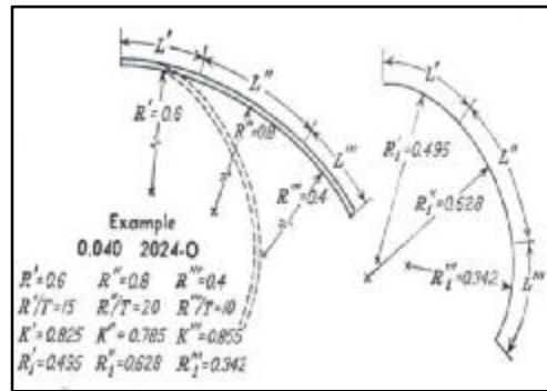
Figure (3) Graphical method determining form- block contours
