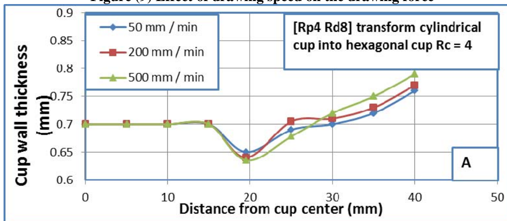
Figure (10) Effect of drawing speed on cup wall thickness
