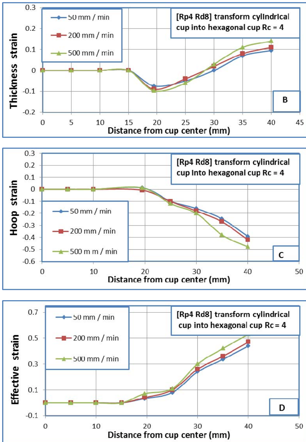
Figure (11) Effect drawing speed on (A) radial strain (B) thickness strain (C) hoop strain (D) effective strain
