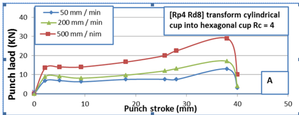
Figure (9) Effect of drawing speed on the drawing force
