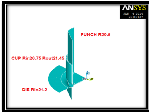
Figure (1) Finite element model of the sheet material and drawing (A) cylindrical die and punch (B) Hexagonal die and punch
