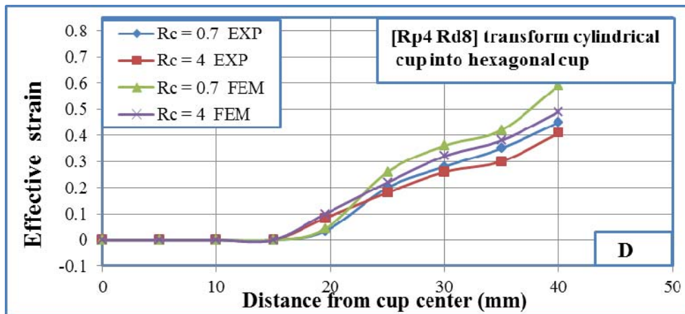
Figure (8) Effect of wall corner radius of die on (A) radial strain (B) thickness strain (C) hoop strain (D) effective strain
