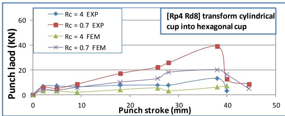
Figure (6) Effect of wall corner radius of die on the drawing force
