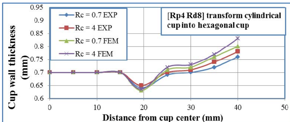
Figure (7) Effect of wall corner radius of die on cup wall thickness
