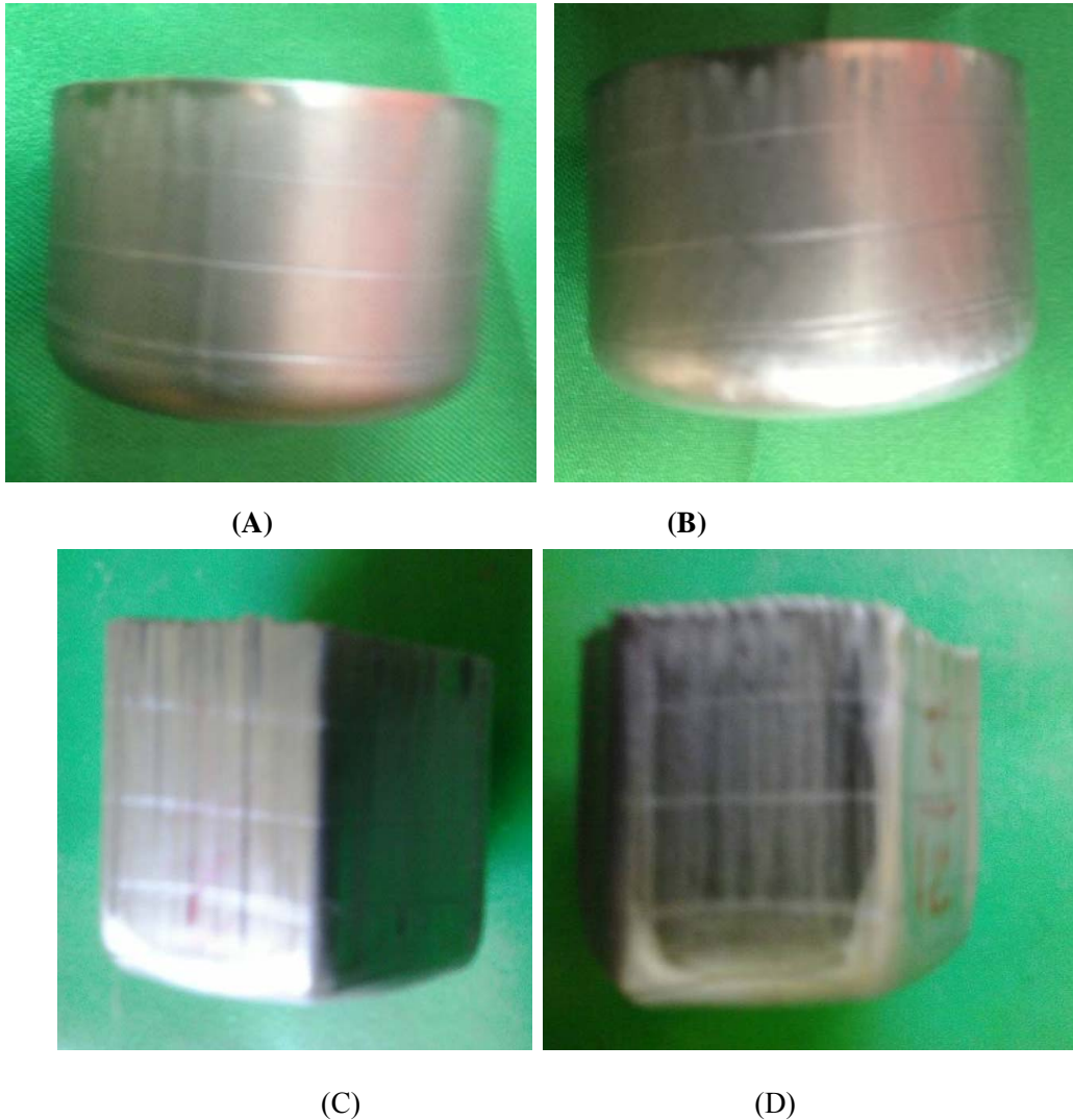
Figure (5) The distortion of grid circles on the (A) (B) cylindrical cup and (C) (D) hexagonal cup from transform cylindrical cup into hexagonal cup.
