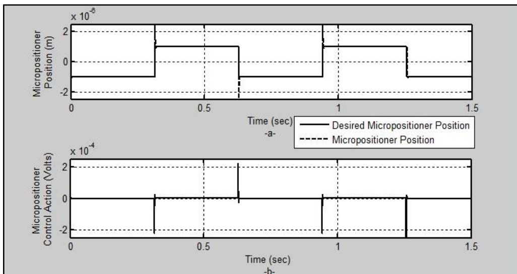
Figure (9) Simulation Results with square function input, magnitude= 1\mu m , frequency= 10\text{ rad/s} a- Time Response. b- Control Action.
