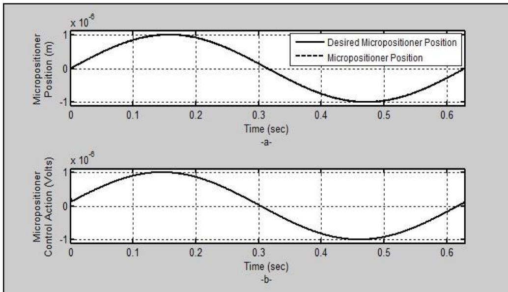
Figure (8) Simulation Results with sinusoidal input, magnitude= 1 \mu m , frequency=10 rad/s a- Time Response. b- Control Action.
