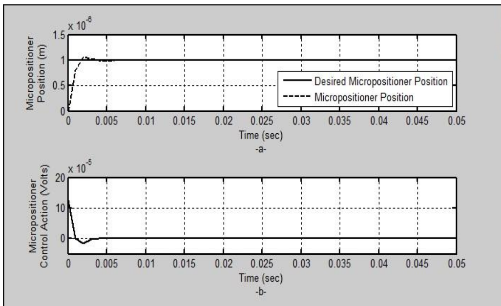
Figure (7) Simulation Results with step input = 1 \mu m a- Time Response. b- Control Action.
