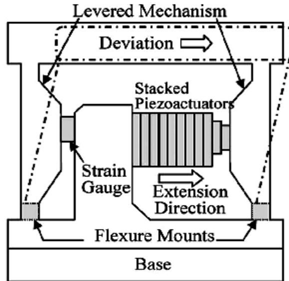
Figure (2) Working Principle of the Piezo-Positioning Stage [4].
