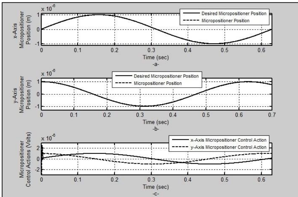
Figure (10) Simulation Results with Sinusoidal Ref. Inputs of Double-Axis Piezoelectric Micropositioner Stage Position. a- Time Response of x-Axis. b- Time Response of y-Axis. c- Double-Axis Control Actions.
