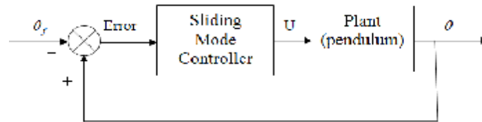
Figure (5): the pendulum system with the Sliding Mode controller.
