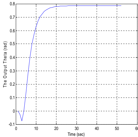
Figure (20): The plot of the output q with time.
