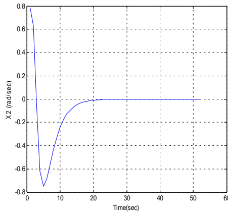
Figure (22): The plot of of x_2 with time.
