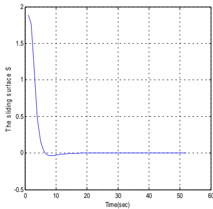
Figure (24): The plot of the Sliding Surface S with time.
