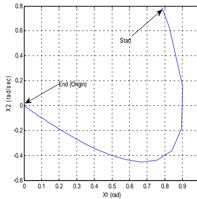
Figure (19): The plot of the phase plane of x_2 against x_1 .
