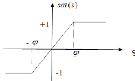
Figure (3): The sat(s) function.
