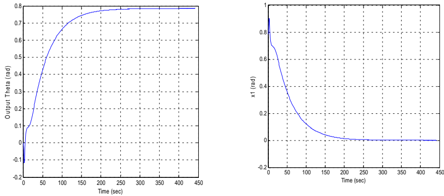
Figure (8): The plot of the output q with time. Figure (9): The plot of the error x_1 with time.
