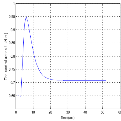
Figure (23): The plot of the control action u with time.
