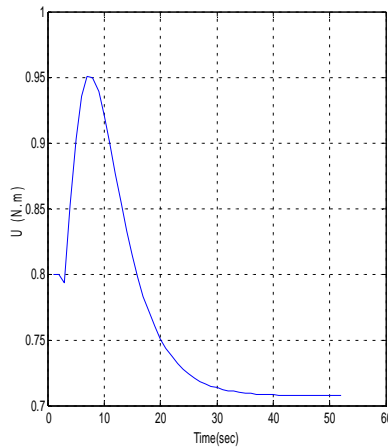
Figure (17): The plot of the control action u with time.
