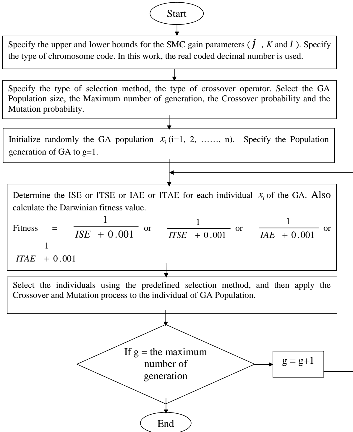
Figure (6): The flow chart of Genetic Algorithm
