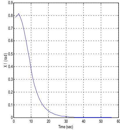
Figure (15): The plot of the error x_1 with time.
