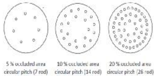
Figure (2) Configuration of internals in bubble column
