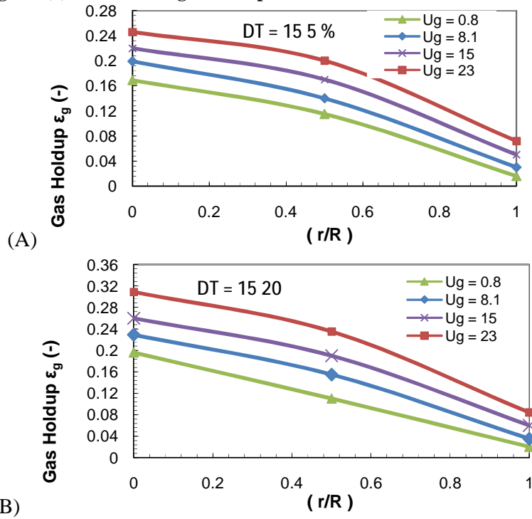
Figure. (7) Radial gas holdup profiles at different superficial gas velocities a) 5% b) 20% internals
