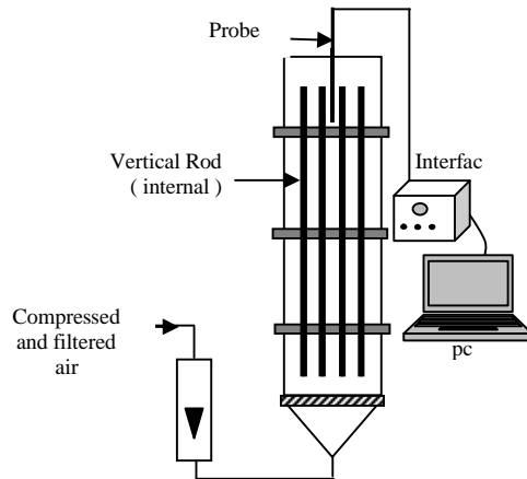
Figure (1) Schematic diagram of bubble column setup
