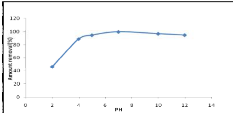
Figure(6) : Adsorption of (JGB) by (PSC) as a function of solution pH at initial concentration of 50 mg/l and adsorbent dosage of 1.5 g with 0.3mm particle size
