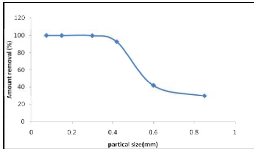
Figure(5) : Effect of particle size on adsorption capacity of (JGB) onto (PSC) at initial dye concentration of 50 mg/l and adsorbent dose of 1.5gm
