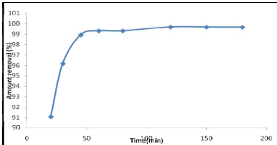
Figure (4) : Effect of contact time for adsorption of (JGB) onto (PSC) at initial dye concentration of 50 mg/l, adsorbent dose of 1.5 g, and particle size of 0.3mm
