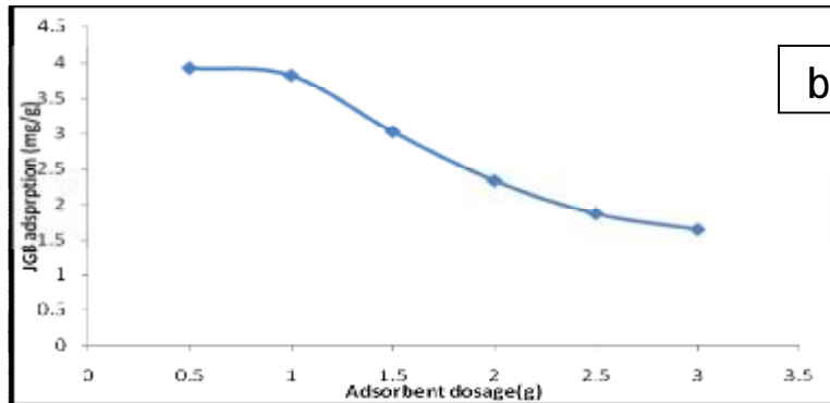
Figure (3 ) Effect of adsorbent dosage in the removal of JGB by (PSC)
