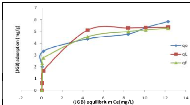
Figure(10): Comparison of experimental and calculated data by Langmuir and Freundlich equilibrium isotherms for the system (JGB) – (PSC)
