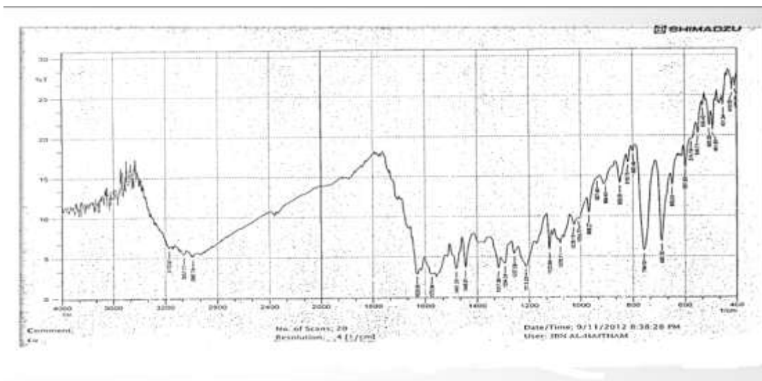
Fig- 4: Infrared spectrum of the [L.CuCl 2 .H 2 O].2H 2 O
