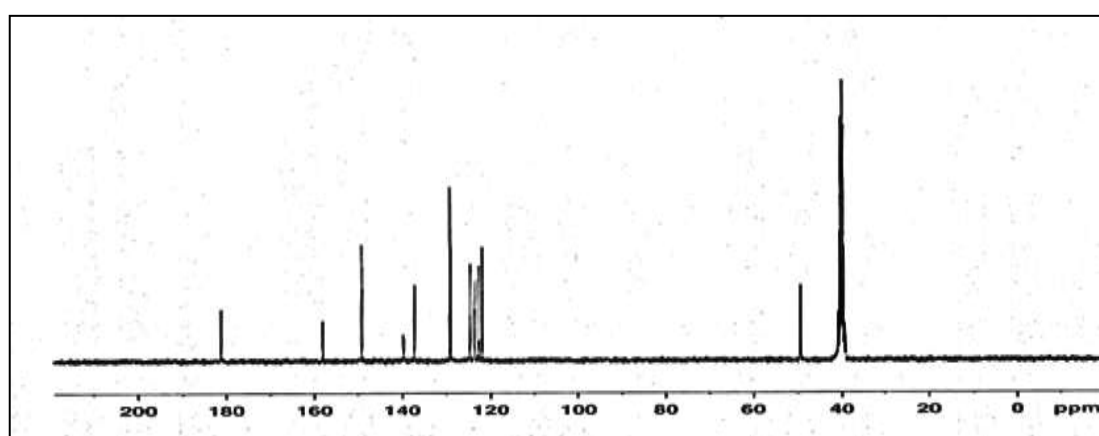
Fig- 2 : 13 C NMR spectrum of the ligand (L)
