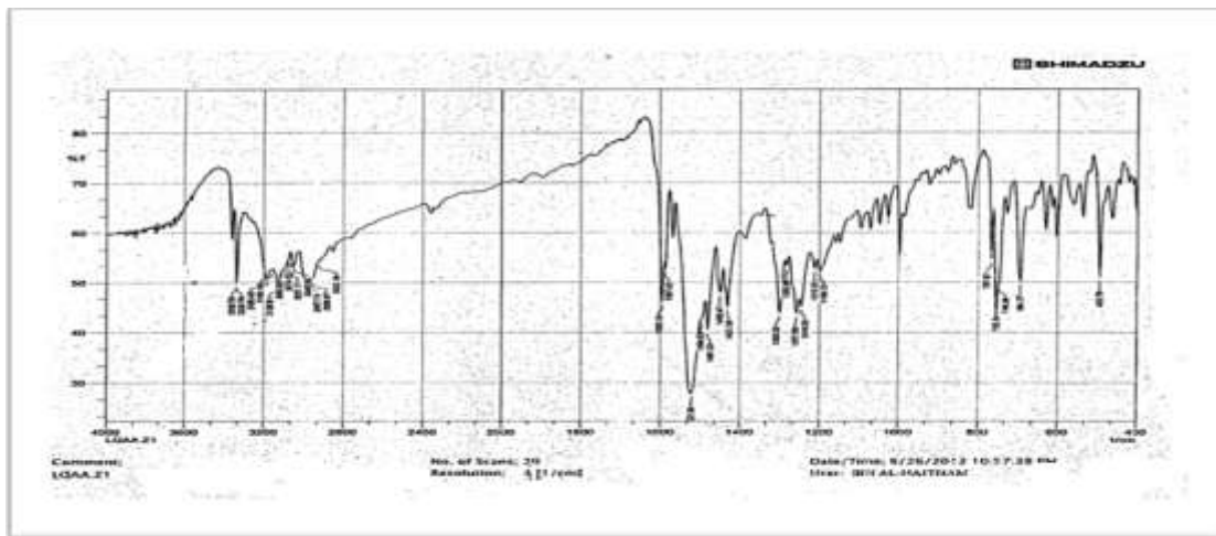
Fig- 3: Infrared spectrum of the ligand(L)
