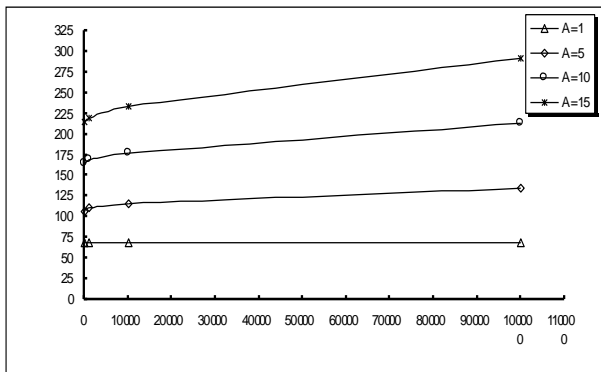
Fig. (7) Variation Nu with the Re for different values of A and (wt) = \pi/2 . Case (I)
