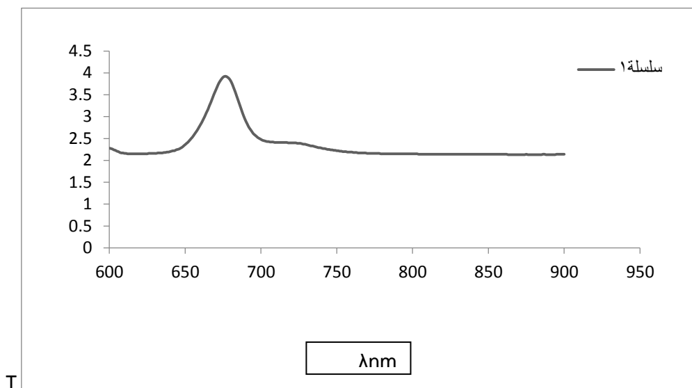
Figure (12) Fluorescence spectrum of the Olive oil
