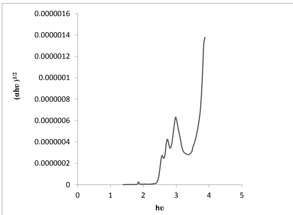
Figure(11)The relationship between the energy and the energy gap
