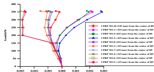
Figure (22) Applied load - CFRP Strain for Beam B9 (21)
