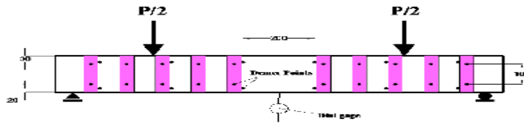
Figure. (8) Details and Instrumentation of Specimen (21)
