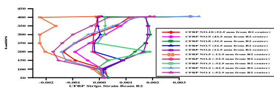
Figure (15) Applied load - CFRP Strain for Beam B2 (21)
