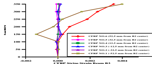
Figure(16) Applied load - CFRP Strain for Beam B3 (21)
