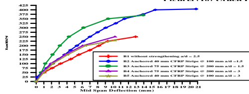
Figure(11): Effect of Varying a/d Ratio on The Load-Deflection of The Beams With Anchorage End CFRP (21)
