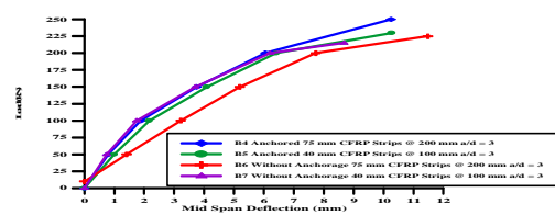
Figure(14): Effect of The CFRP End Anchorage on the Load-Deflection of The Beams With (a/d = 3) (21)
