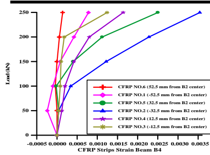
Figure (17) Applied load - CFRP Strain for Beam B4 (21)
