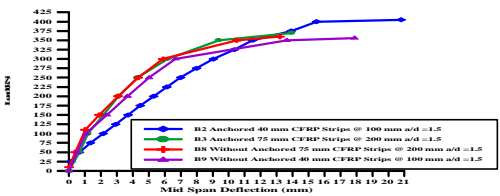
Figure(13): Effect of The CFRP End Anchorage on the Load-Deflection of The Beams With (a/d = 1.5) (21)
