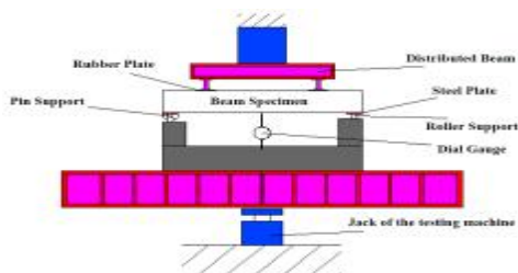
Figure (7) Beams Testing Machine Details (21)
