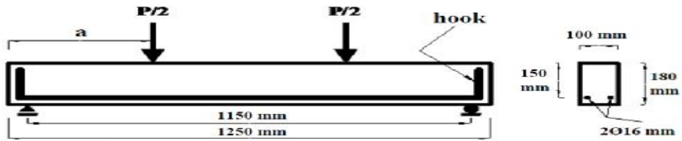
Figure (1) Details of Typical Tested Beams (21)
