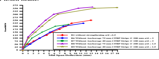
Figure(12): Effect of Varying a/d Ratio on The Load-Deflection of The Beams Without Anchorage End CFRP (21)
