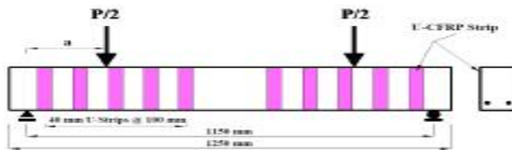
Figure (5) Shear Strengthening without End Anchoring B7 and B9 (21)
