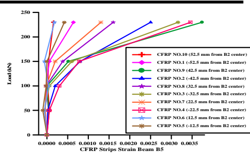
Figure (18) Applied load - CFRP Strain for Beam B5 (21)
