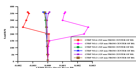
Figure (21) Applied load - CFRP Strain for Beam B8 (21)
