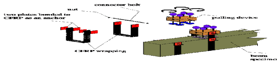
Figure (2) Details of Preparing and Fixing System of the U-wrap CFRP and Devices (21)
