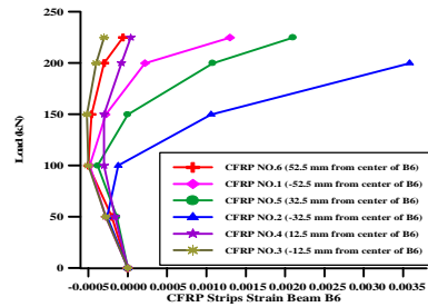
Figure (19) Applied load - CFRP Strain for Beam B6 (21)
