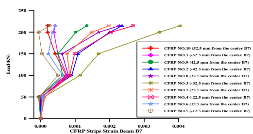
Figure (20) Applied load - CFRP Strain for Beam B7 (21)
