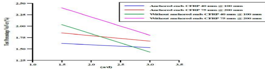
Figure(9): Effect of (a/d) Ratio on the Percentage Decrease in Shear Strength of SFRHSC Beams (21).
