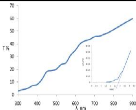
Figure (2) Optical transmission spectra of CdS nanoparticles.
