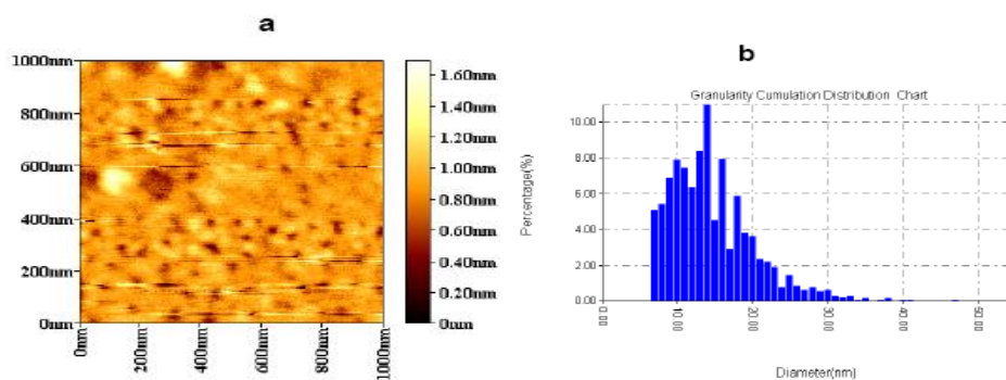
Figure (3) AFM image of CdS nanoparticles; a) two dimensional image. b) Histogram of crystal size distribution.
