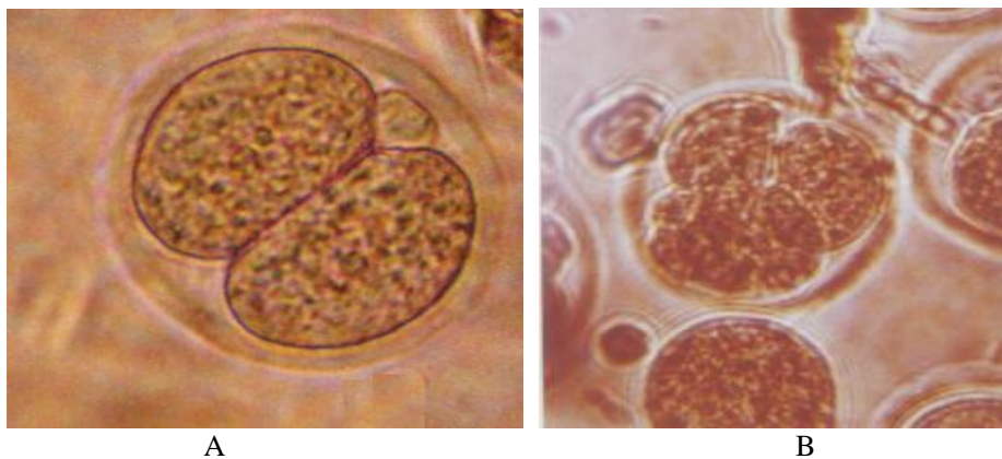
Figure (3) cleaved oocyte by IVF. (A) 2 cells embryo, (B) 4 cells embryo. (X 10).
