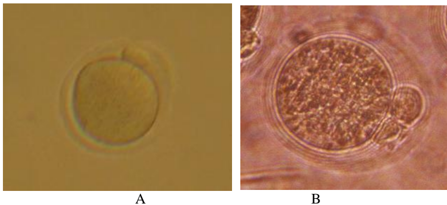
Figure (2) matured oocyte (A) and fertilized oocyte (B) (X 10).
