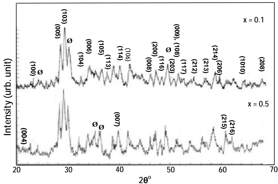
Figure (1) XRD pattern of Cu-doped Hg_{1-x}Cu_xBa_2Ca_2Cu_3O_{8+\delta} With x oncentration 0.1 and 0.5.
