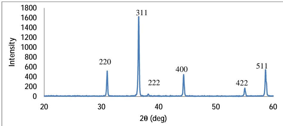
Figure (6): XRD patterns of NiFe 2-x Al x O 4 samples sintered at 1200°C
