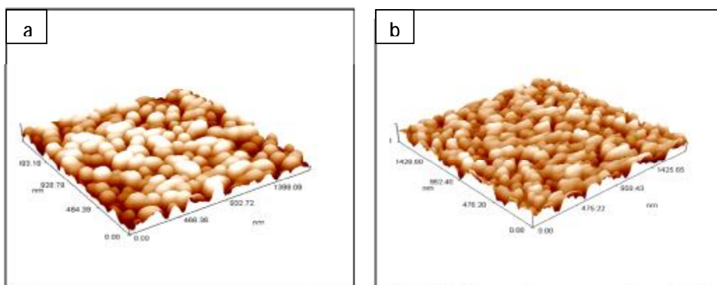
Figure (8): Surface morphology 3D image (a) AFM for as-burnt powder at 200 °C (b) AFM for calcined sample at 500 °C for \text{NiFe}_{2-x}\text{Al}_x\text{O}_4 ferrite nanopowders
