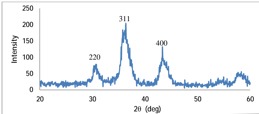
Figure (2): XRD patterns of ( \text{NiFe}_{2-x}\text{Al}_x\text{O}_4 ) powder calcined at 500° C
