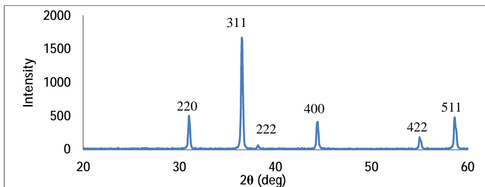
Figure (5): XRD patterns of \text{NiFe}_{2-x}\text{Al}_x\text{O}_4 samples sintered at 1100°C
