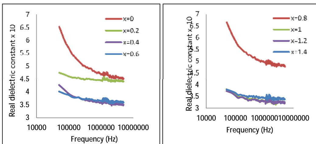
Figure (9): Variation of the real dielectric constant with frequency of \text{NiAl}_x\text{Fe}_{2-x}\text{O}_4 With ( x=0.0 - 1.4 ) sintered at temp. 1200^\circ\text{C}
