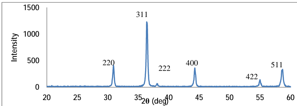
Figure (3): XRD patterns of (\text{NiFe}_{2-x}\text{Al}_x\text{O}_4) samples sintered at 900°C
