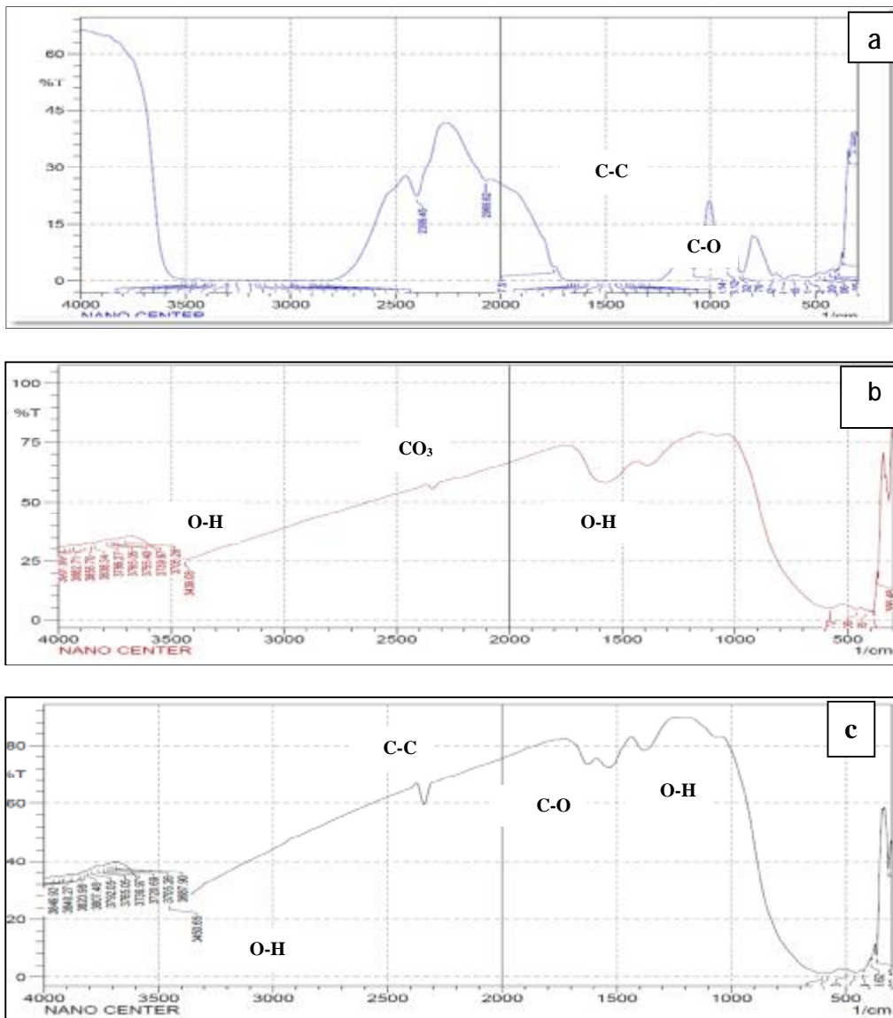
Figure (7) : FTIR spectra of; (a) dry gel at 110 °C, (b) as-burnt powder at 200 °C, (c) Calcined powder at 500 °C of (\text{NiFe}_{2-x}\text{Al}_x\text{O}_4) nanoferrite
