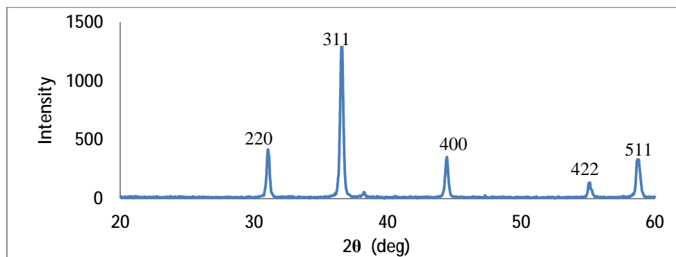
Figure (4): XRD patterns of (\text{NiFe}_{2-x}\text{Al}_x\text{O}_4) samples sintered at 1000°C
