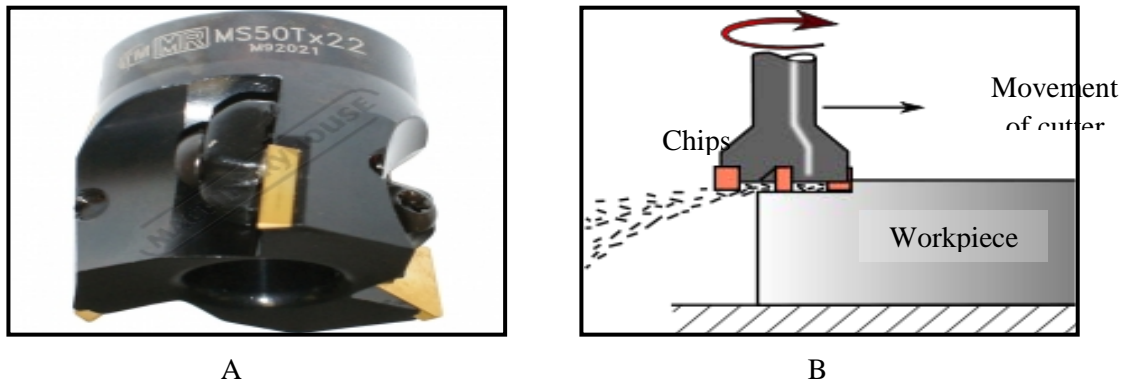
Figure (2) show: (A) face milling tool and, (B) face milling process.
