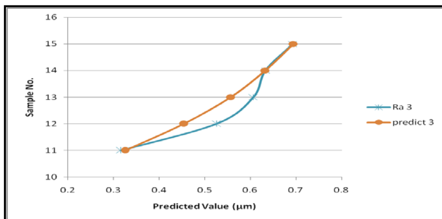
Figure (10) Relationship between real and predicted values at third stage of experiments.
