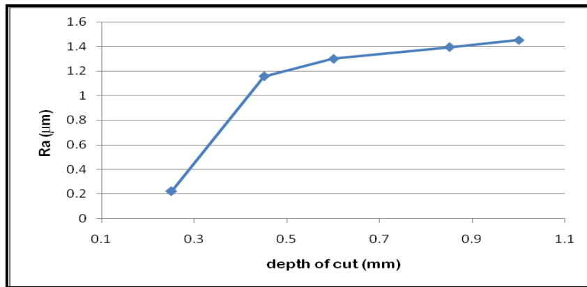
Figure (6) Effect of depth of cut on surface roughness.
