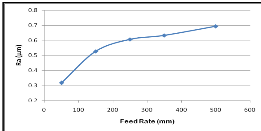
Figure (7) Effect of feed rate on surface roughness
