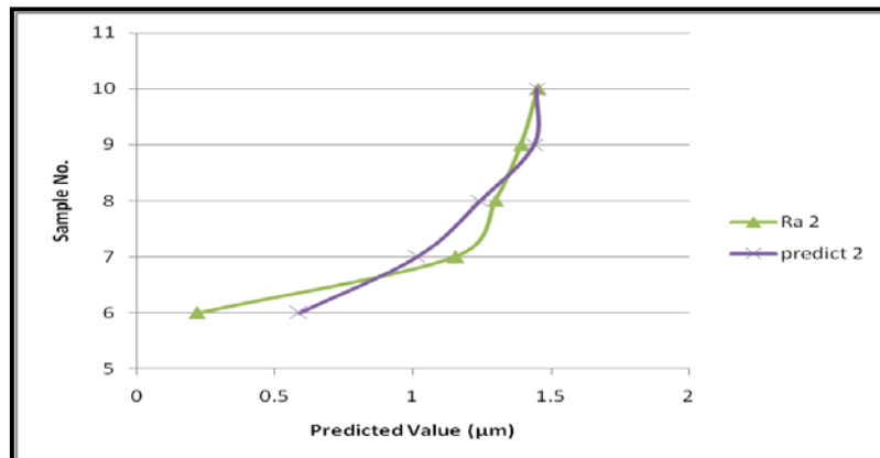
Figure (9) Relationship between real and predicted values at second stage of experiment.
