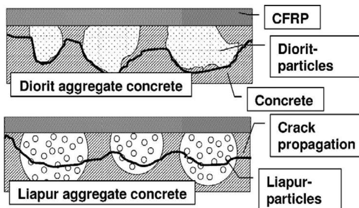
Figure( 2-b) Difference in crack propagation for different bonding qualities[3].
