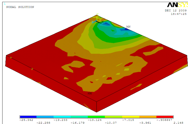
Figure.(5) Crack patterns for slab specimen (SL) (bottom view)
