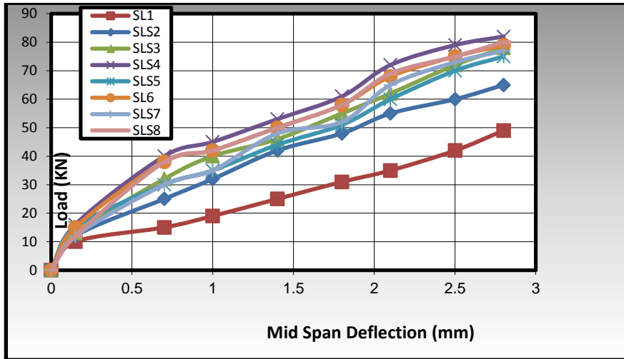
Figure (4) Load versus mid-span deflection
