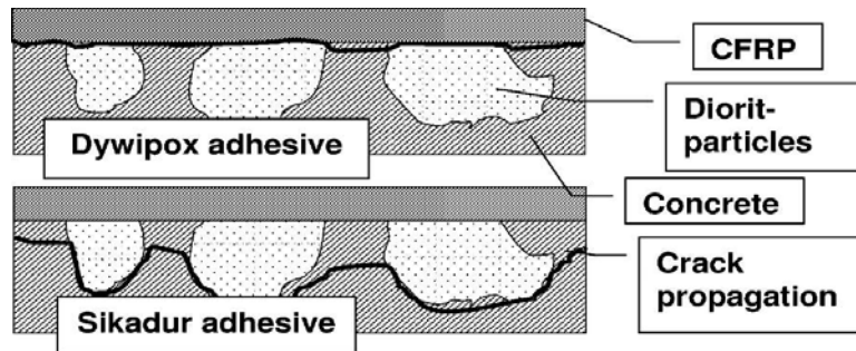
Figure(2-a) Difference in crack propagation for strong and weak aggregate types[ 3].
