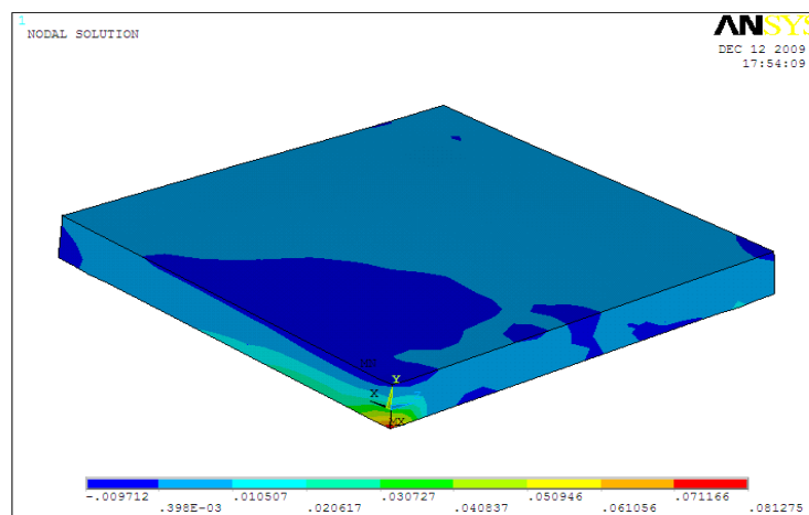
Figure (7) Variations in strain in Z-direction for control slab (LC)
