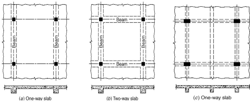
Figure (1): Several cases of one-way slab and two-way slab[1].
