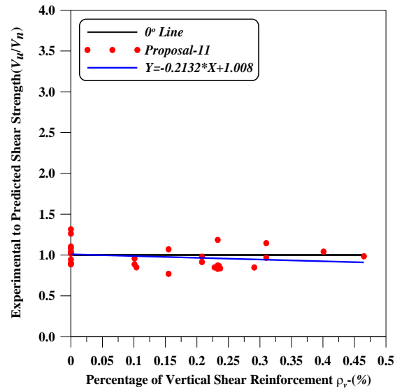
Figure 17: Percentage of Vertical Shear Reinforcement \rho_v versus Ratio of Experimental to Predicted Shear Strengths- ( V_u/V_n )
