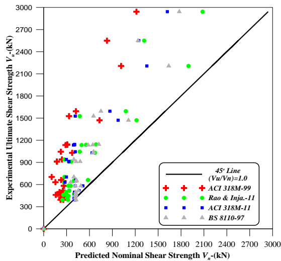
Figure 8: Comparison between Experimental V_u and Empirical- V_n Results
