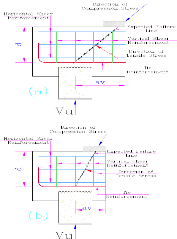
Figure 10: Shear Failure Line Intersecting Shear Reinforcement and Direction of Stresses for; (a) Low ( a_v/d ), (b) High ( a_v/d )
