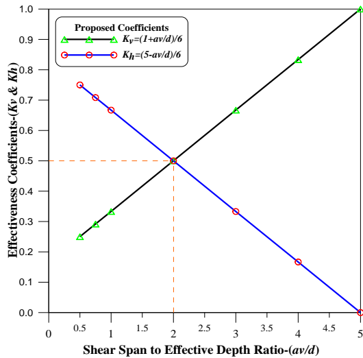
Figure 9: Proposed Effectiveness Coefficients for Vertical & Horizontal Transverse Shear Reinforcements
