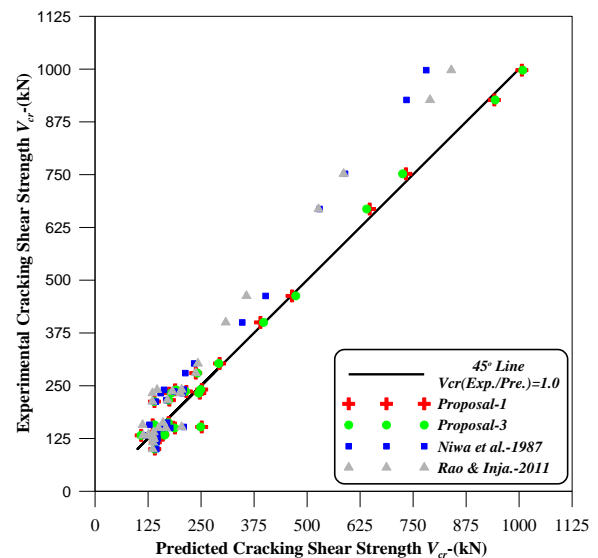
Figure 3: Comparison between Experimental and Predicted Cracking Shear Strength- V_{cr} for Existing and Proposed Equations
