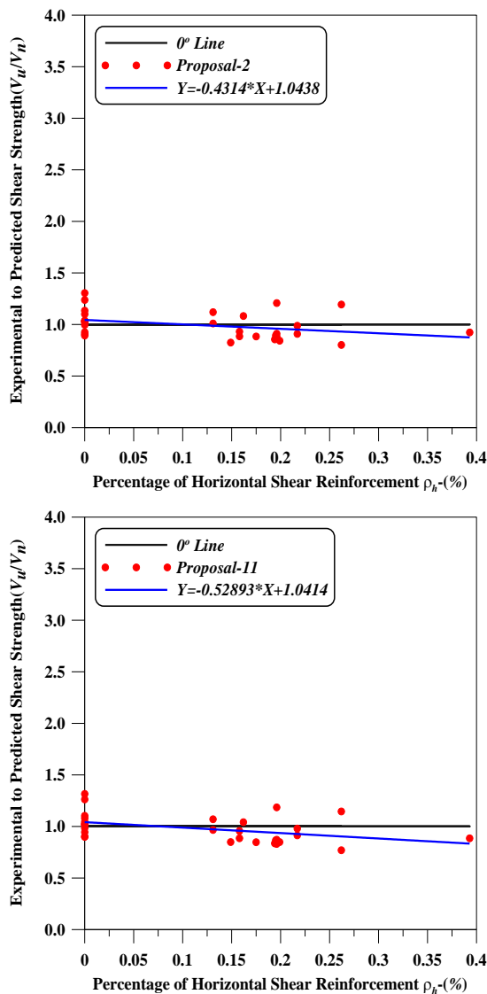
Figure 18: Percentage of Horizontal Shear Reinforcement \rho_h versus Ratio of Experimental to Predicted Shear Strengths- ( V_u/V_n )
