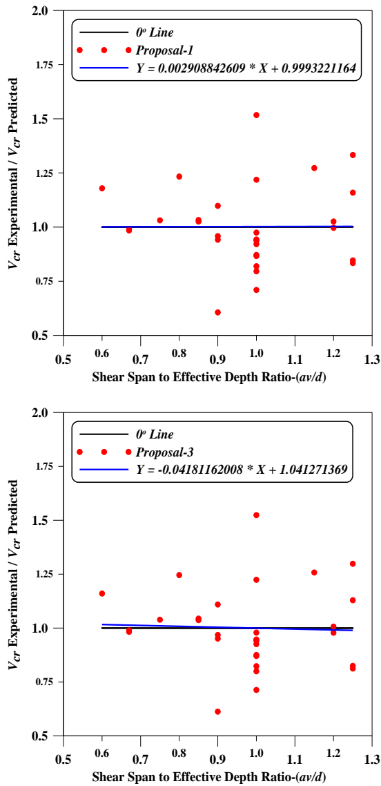
Figure 6: Shear Span to Effective Depth Ratio ( av/d ) versus Ratio of Experimental to Predicted Diagonal Shear Strengths- V_{cr}
