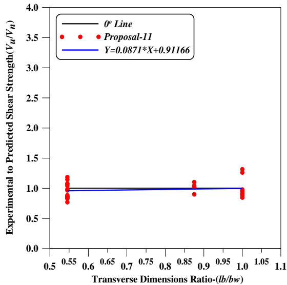
Figure 16: Transverse Dimensions Ratio between Pile and Cap ( lb/bw ) versus Ratio of Experimental to Predicted Shear Strengths- ( V_u/V_n )
