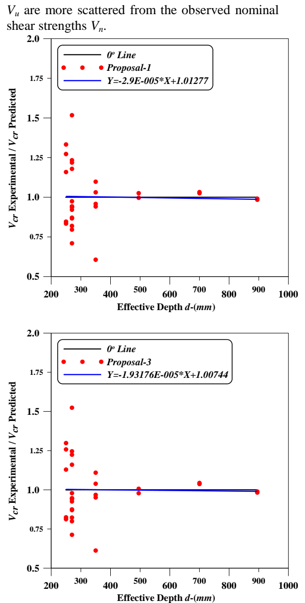
Figure 7: Effective Depth d versus Ratio of Experimental to Predicted Diagonal Shear Strengths- V_{cr}
