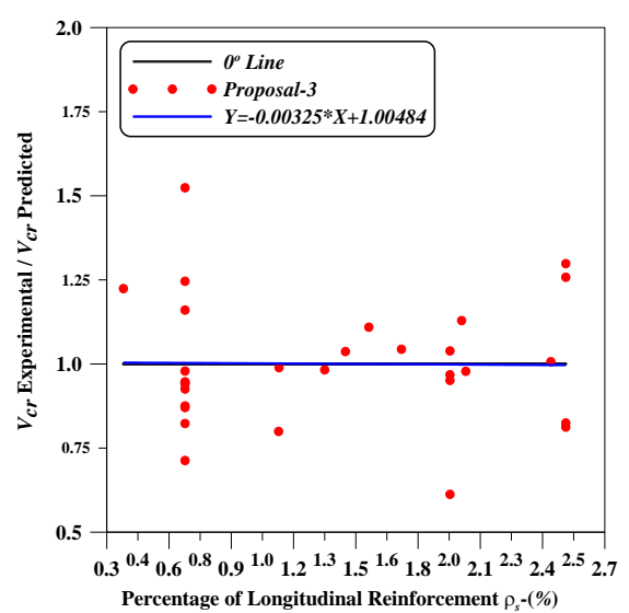
Figure 5: Percentage of Longitudinal Reinforcement \rho_s versus Ratio of Experimental to Predicted Diagonal Shear Strengths- V_{cr}
