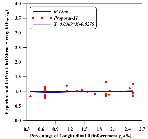
Figure 13: Percentage of Longitudinal Reinforcement \rho_s versus Ratio of Experimental to Predicted Shear Strengths- (V_u/V_n)
