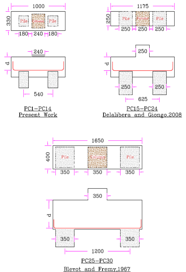
Figure 1: Pile Caps Geometry and Section for Use in Statistical Analysis
