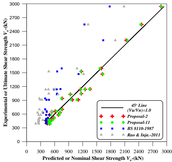
Figure 11: Comparison between Experimental V_u and Predicted V_n Shear Strength
