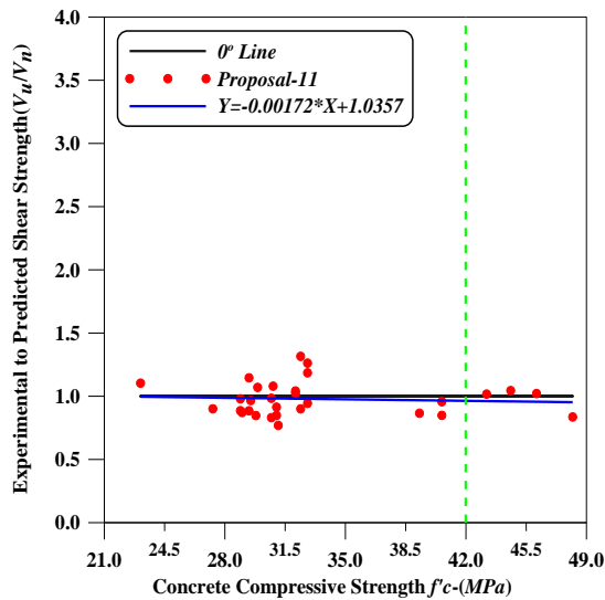
Figure 12: Concrete Compressive Strength f_c versus Ratio of Experimental to Predicted Shear Strengths- (V_u/V_n)
