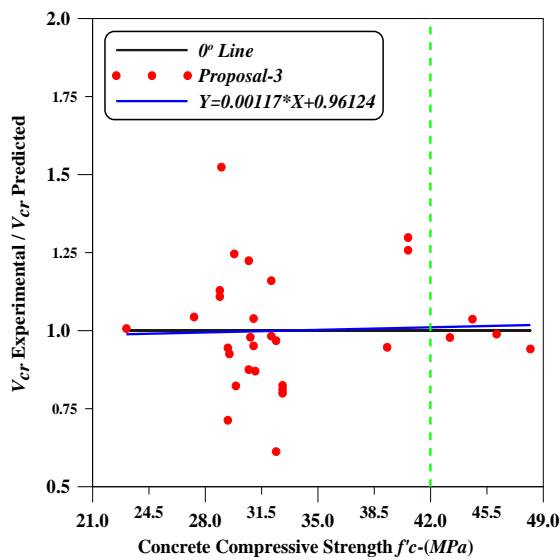
Figure 4: Concrete Compressive Strength f'c versus Ratio of Experimental to Predicted Cracking Shear Strengths- V_{cr}
