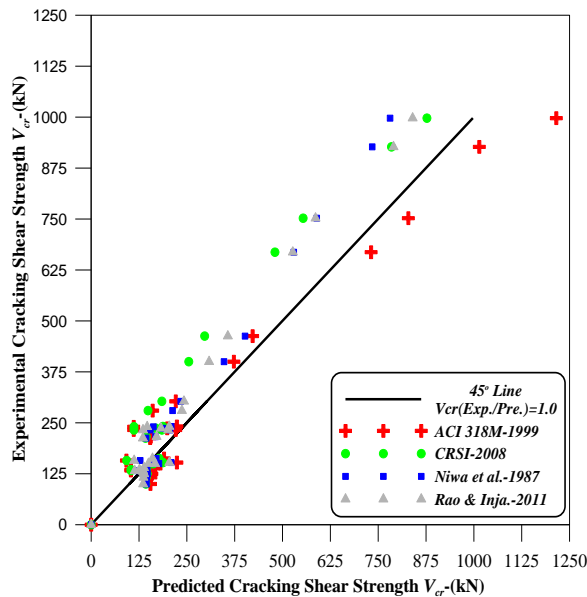
Figure 2: Comparison between Experimental and Empirical Results- V_{cr}
