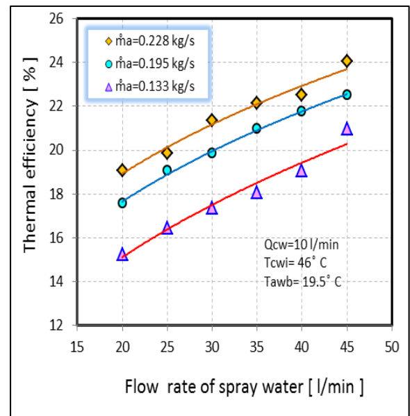
Figure 4: Variation of thermal efficiency with spray water flow rate for different air flow rates
