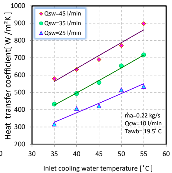
Figure 14: Variation of heat transfer coefficient with inlet cooling water temperature for different spray water flow rates
