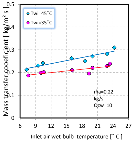
Figure 17: Variation of mass transfer coefficient with inlet AWBT for different inlet water temperatures
