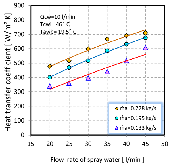
Figure 6: variation of heat transfer coefficient with spray water flow rate for different air flow rates
