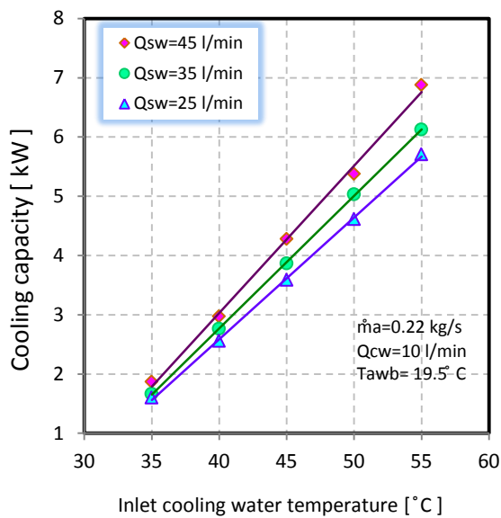
Figure 11: Variation of cooling capacity with inlet cooling water temperature for different spray water flow rates
