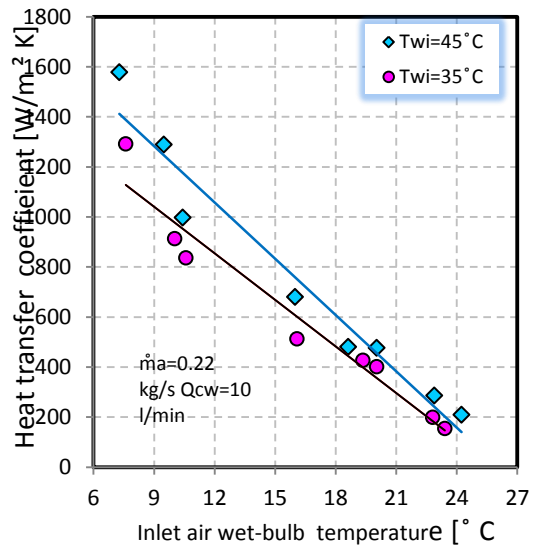
Figure 18: Variation of heat transfer coefficient with inlet AWBT for different inlet water temperatures
