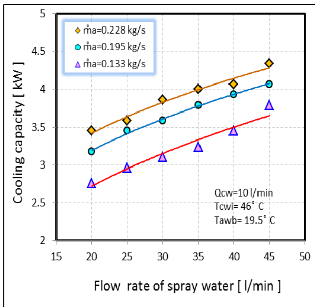
Figure 3: variation of cooling capacity with spray water flow rate for different air flow rates
