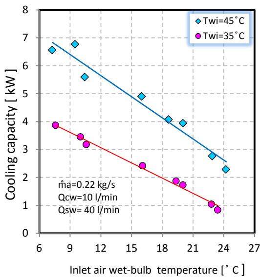
Figure 15: Variation of cooling capacity with inlet AWBT for different inlet water
