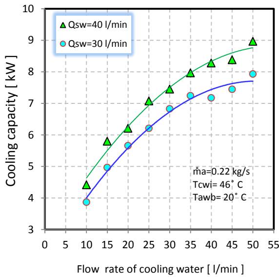
Figure 7: variation of cooling capacity with cooling water flow rate for different spray water flow rates
