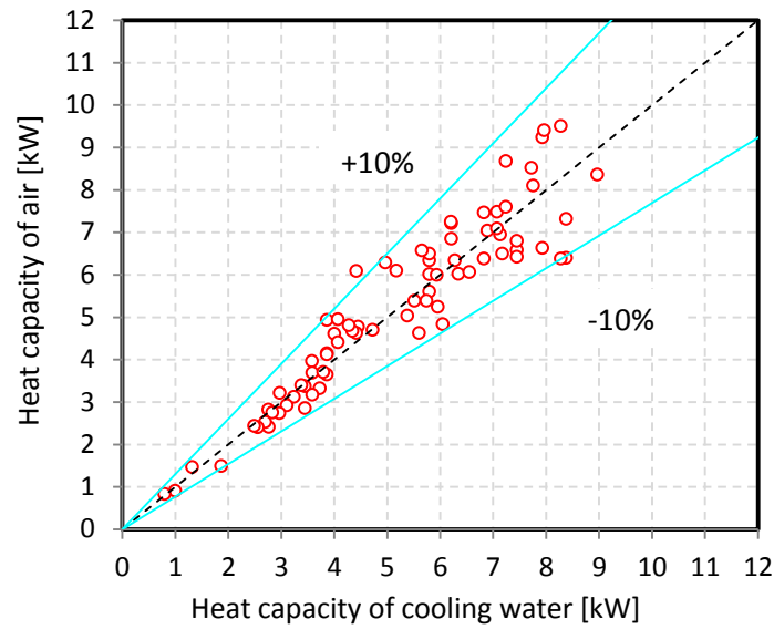
Figure 2: Energy balance of the experimental apparatus
