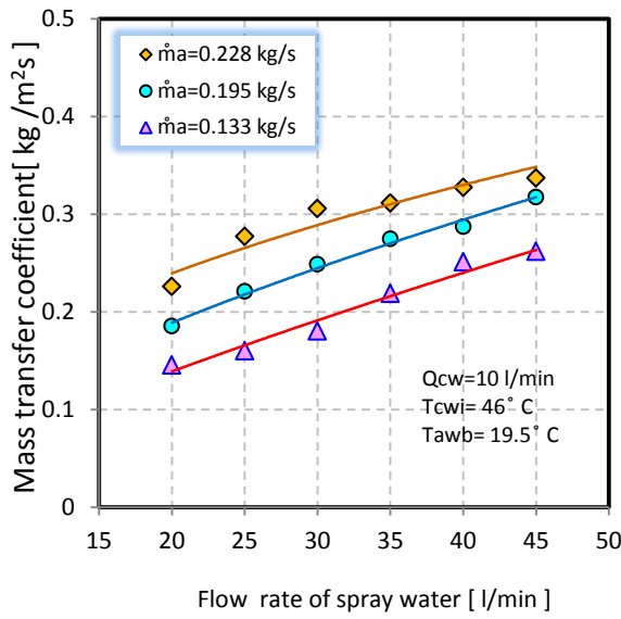
Figure 5: Variation of mass transfer coefficient with spray water flow rate for different air flow rates
