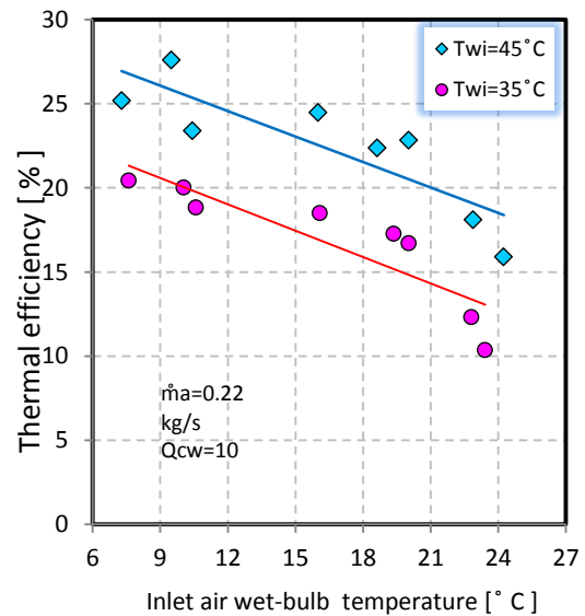
Figure 16: Variation of thermal efficiency with inlet AWBT for different inlet water temperatures
