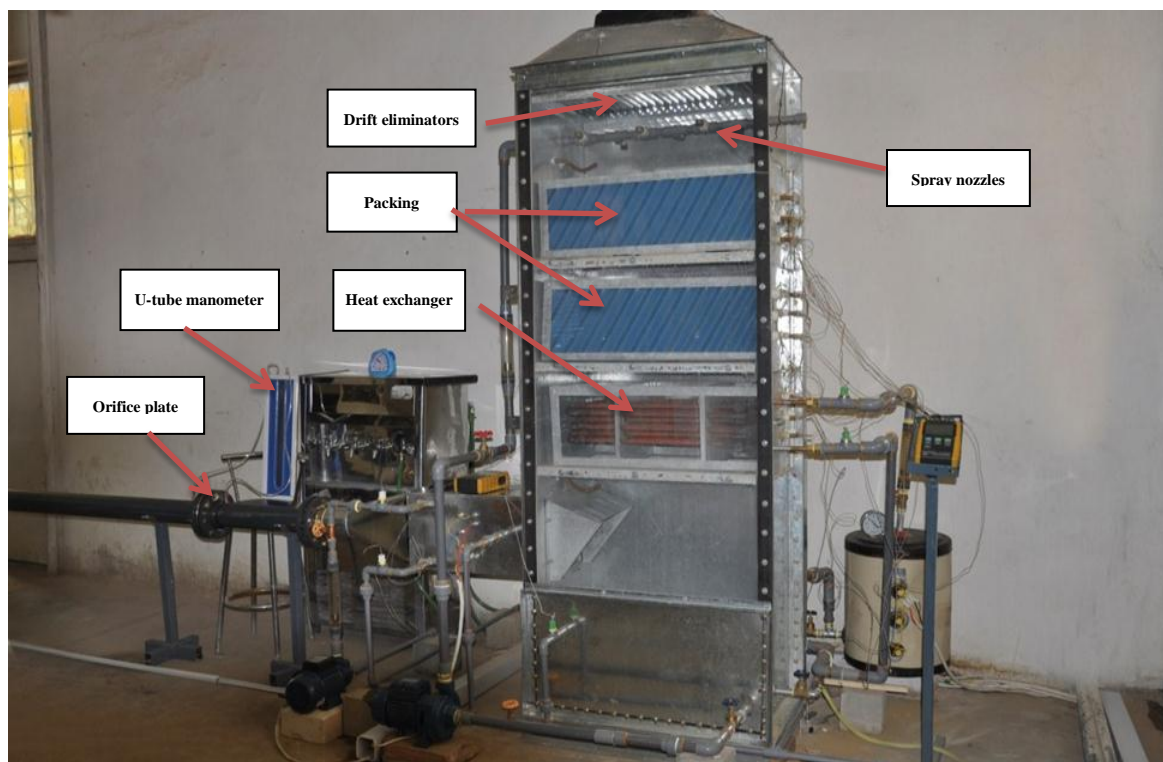
Figure 1b: Photographic picture for experimental apparatus (front view)
