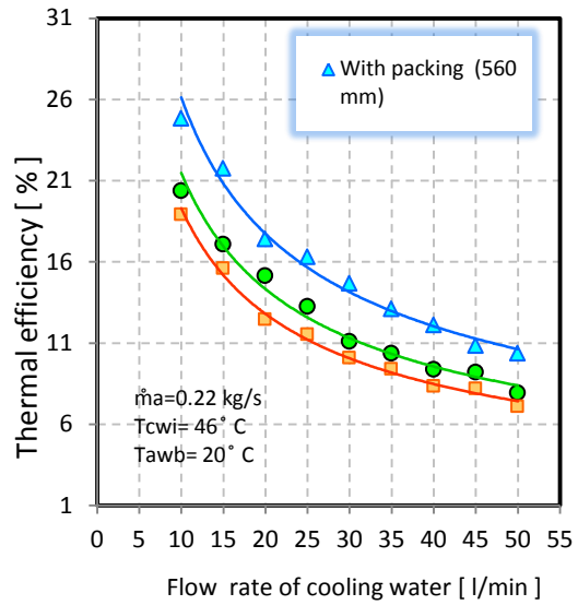
Figure 20: Variation of thermal efficiency with cooling water flow rate for different heights of packing
