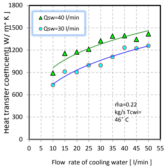
Figure 10: Variation of heat transfer coefficient with cooling water flow rate for different spray water flow rates
