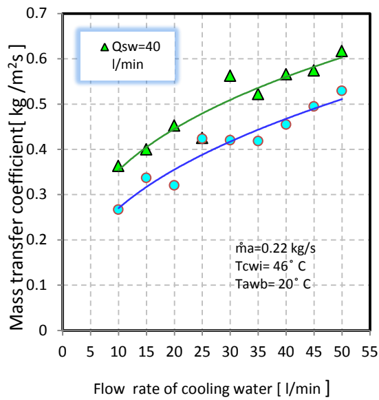
Figure 9: Variation of mass transfer coefficient with cooling water flow rate for different spray water flow rates
