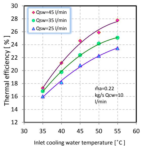
Figure 12: Variation of thermal efficiency with inlet cooling water temperature for different spray water flow rates
