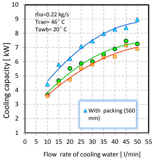
Figure 19: Variation of cooling capacity with cooling water flow rate for different heights of packing
