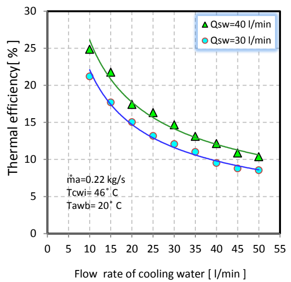
Figure 8: Variation of thermal efficiency with cooling water flow rate for different spray water flow rates
