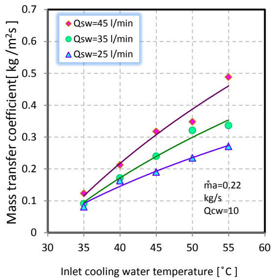
Figure 13: Variation of mass transfer coefficient with inlet cooling water temperature for different inlet water temperatures
