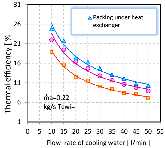
Figure 22: Variation of thermal efficiency with cooling water flow rate for different locations of packing
