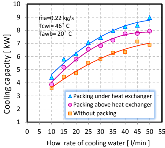
Figure 21: Variation of cooling capacity with cooling water flow rate for different locations of packing
