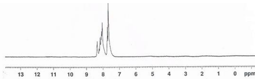
Figure 1: 1 H NMR Spectrum for compound 1,4-di(5-(phenyldiazenyl)-1,3,4-thiadiazol-2-yl)benzene [2]
