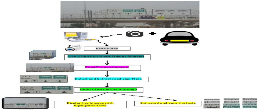
Figure (1) Graphical chart of the algorithm
