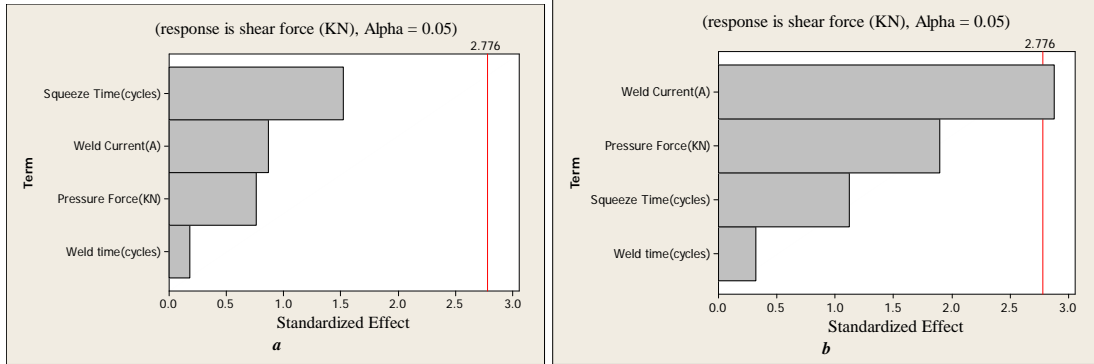
Figure (14) Pareto chart of similar joints for AISI 304L, (a) t = 0.5 mm (b) t = 0.7 mm
