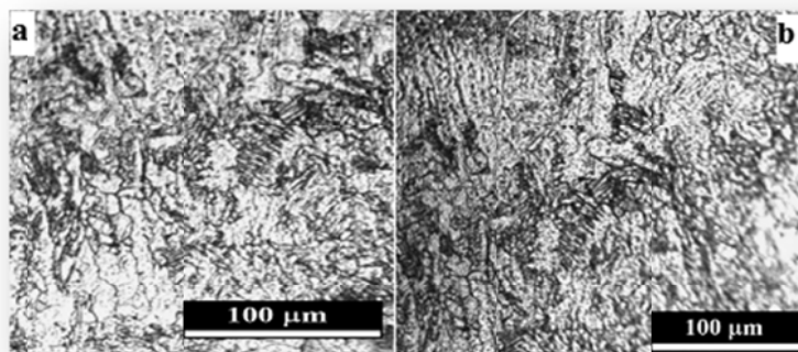
Figure (23) Microstructure of similar joint of AISI 304L, (a) t = 0.5 mm (b) t = 0.7 mm
