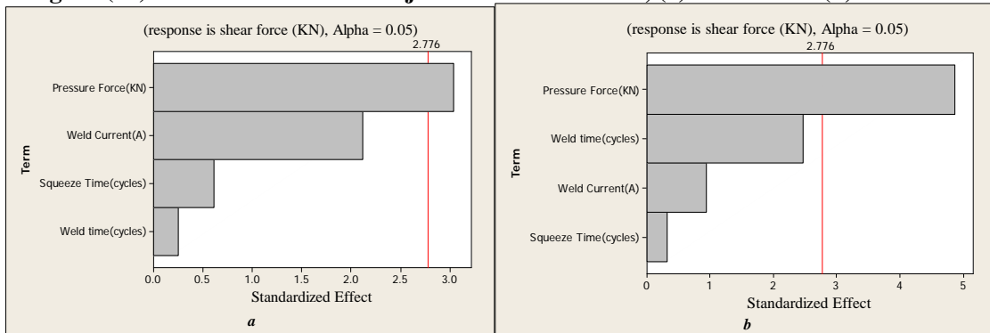
Figure (15) Pareto chart of similar joints for AA 6061-T6, (a) t = 0.5 mm (b) t = 0.7 mm
