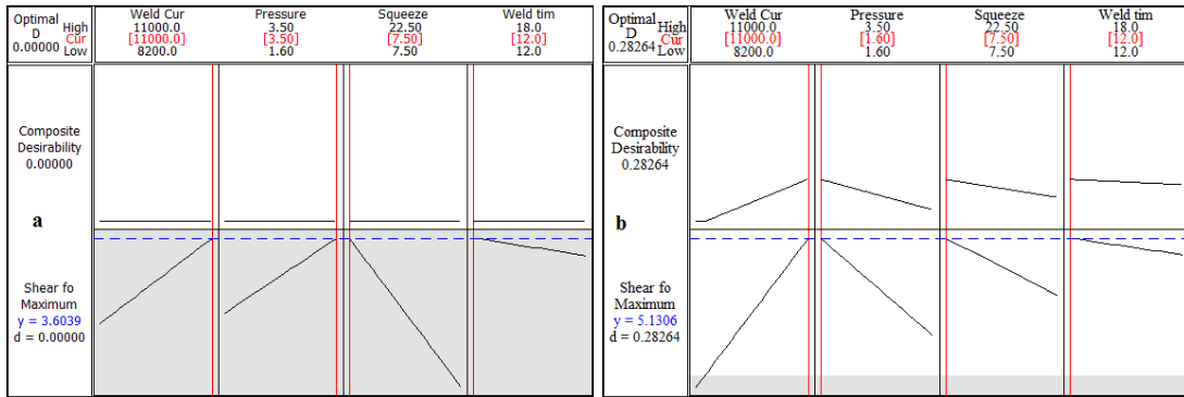
Figure.(17) Response optimizer of similar joints for AISI 304L, (a) t = 0.5 mm (b) t = 0.7 mm
