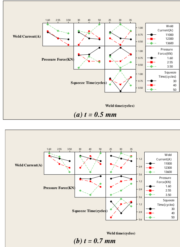
Figure (13) Interactions plot of shear force for dissimilar joints for AISI 304L with AA 6061-T6
