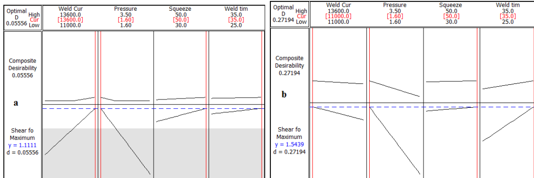
Figure.(19) Response optimizer of dissimilar joints for AISI 304L-AA 6061-T6 , (a) t = 0.5 mm (b) t = 0.7 mm
