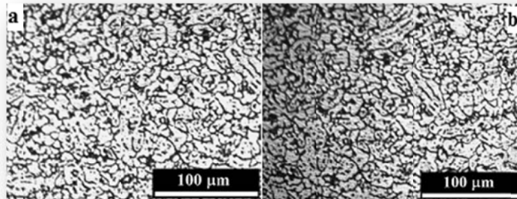
Figure (24) Microstructure of similar joint of AA 6061-T6, (a) t = 0.5 mm (b) t = 0.7 mm
