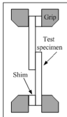
Figure (4) Schematic of tensile strength test
