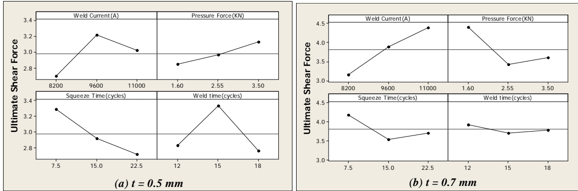
Figure.(8) Main effects plot of shear force for similar joints of AISI 304L
