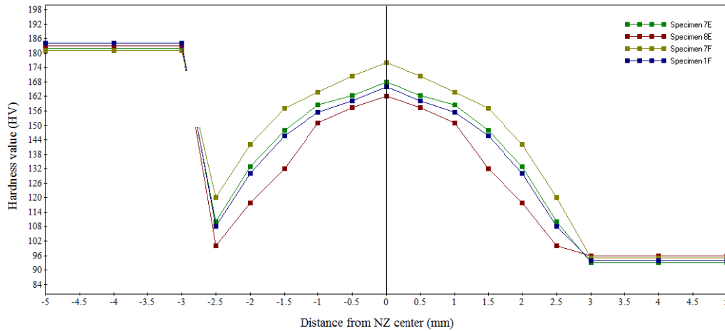
Figure (22) Hardness values of dissimilar joint for (AISI 304L with AA 6060-T6)
