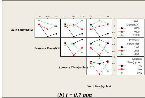
Figure (11) Interactions plot of shear force for similar joints of AISI 304L
