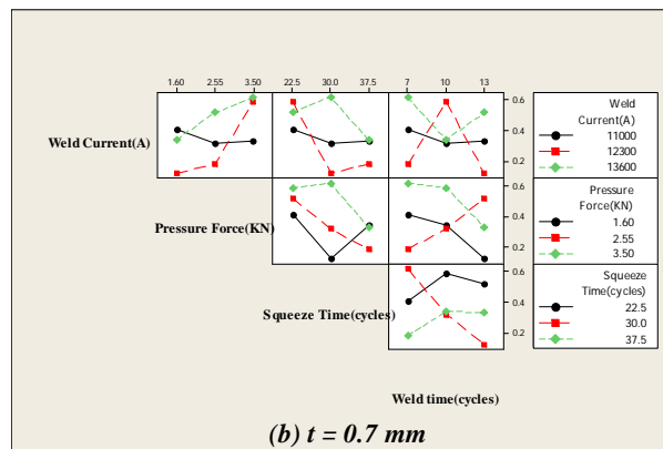
Figure (12) Interactions plot of shear force for similar joints of AA 6061-T6
