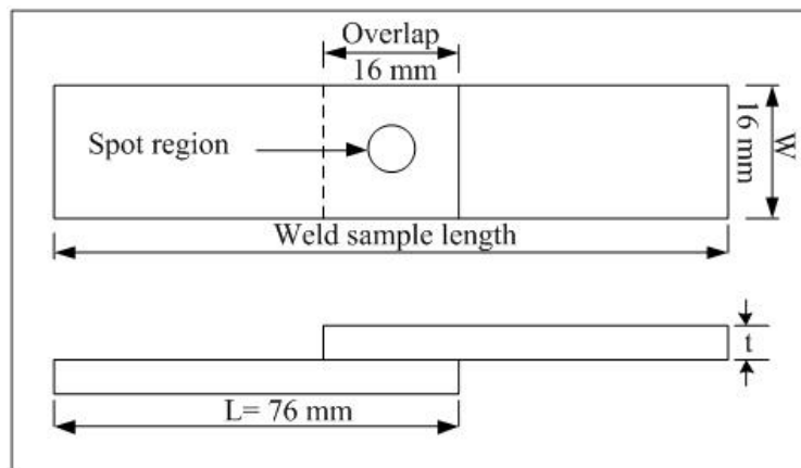
Figure (1) Overlapping of two welded plates
