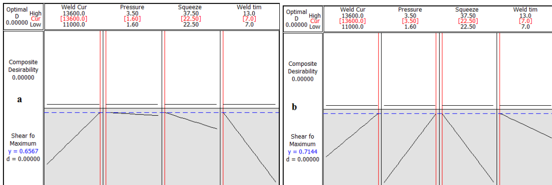
Figure.(18) Response optimizer of similar joints for AA 6061-T6, (a) t = 0.5 mm (b) t = 0.7 mm
