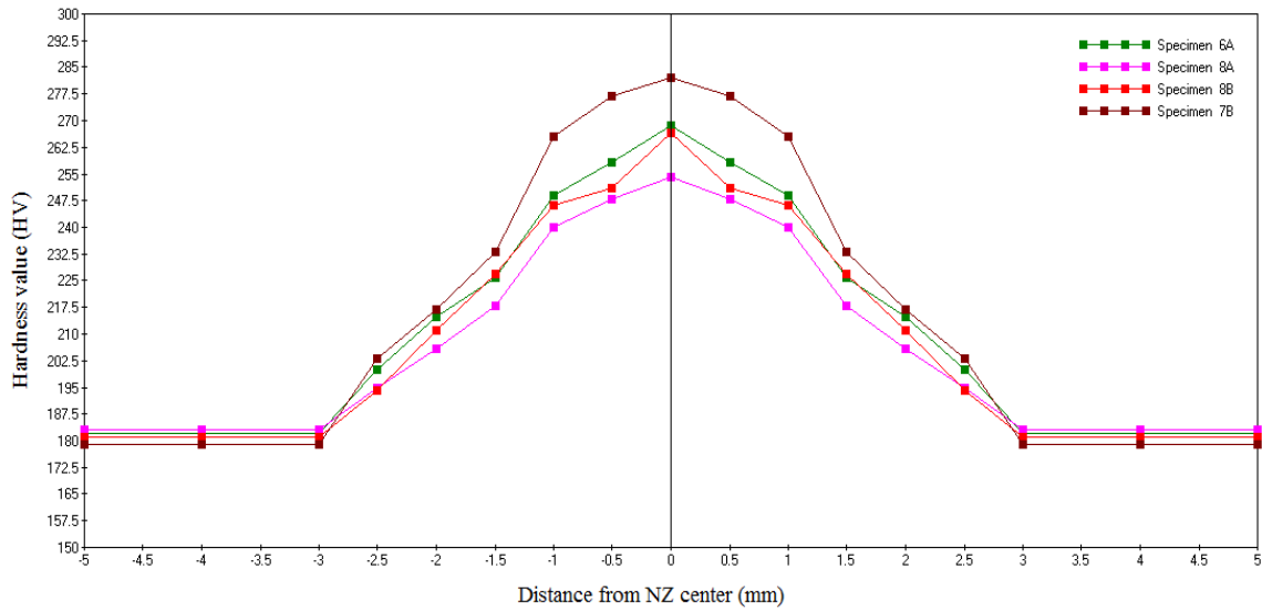
Figure (20) Hardness values of similar joint for AISI 304L
