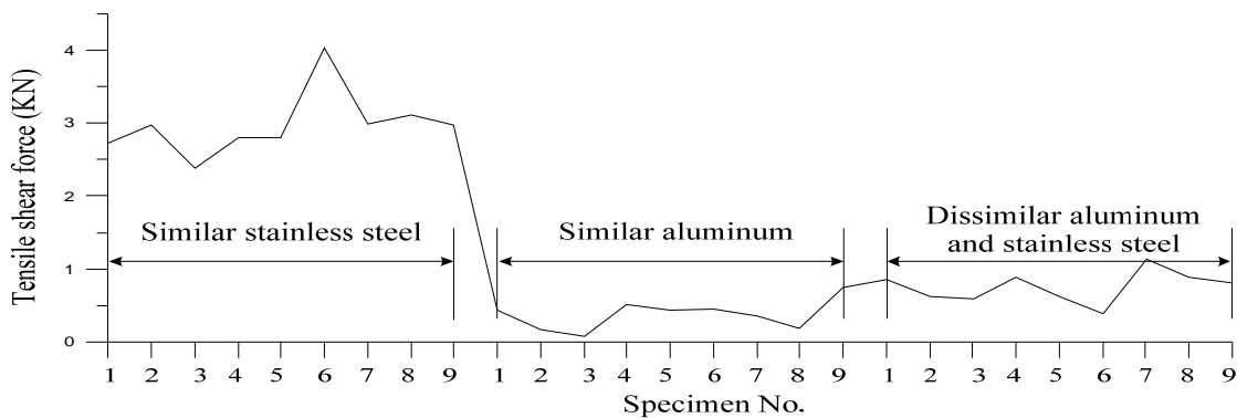
Figure (6) shear force of the welded specimen with thickness (t=0.5 mm)
