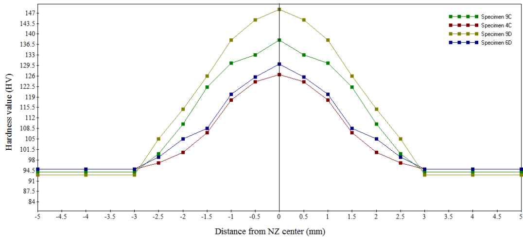
Figure (21) Hardness values of similar joint for AA 6061-T6
