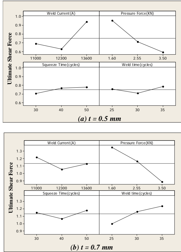
Figure.(10) Main effects plot of shear force for dissimilar joints of AISI 304L with AA 6061-T6
