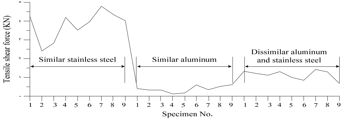
Figure (7) shear force of the welded specimen with thickness (t=0.7 mm)
