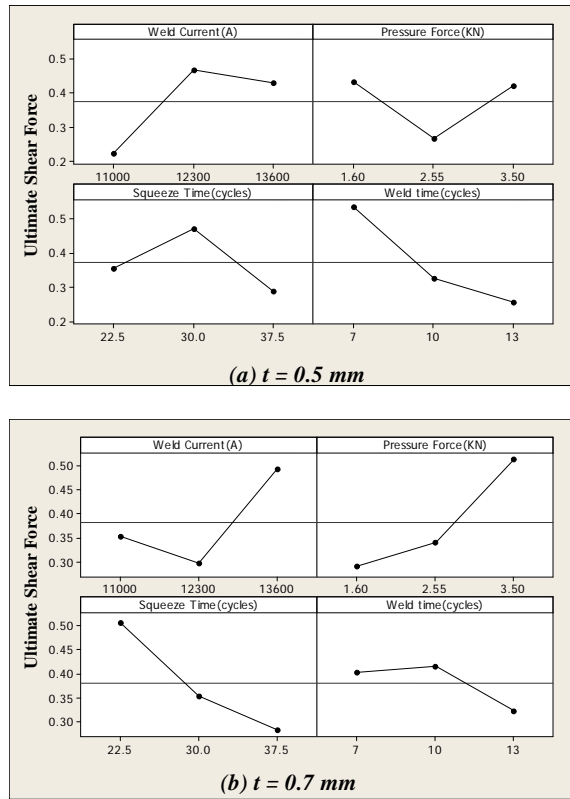
Figure.(9) Main effects plot of shear force for similar joints of AA 6061-T6
