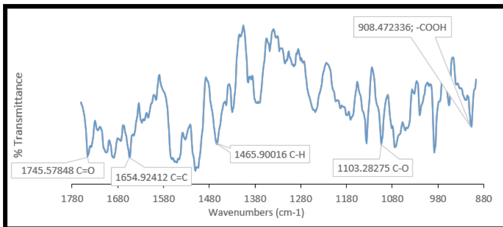
Figure (5): FTIR of functionalized graphene
