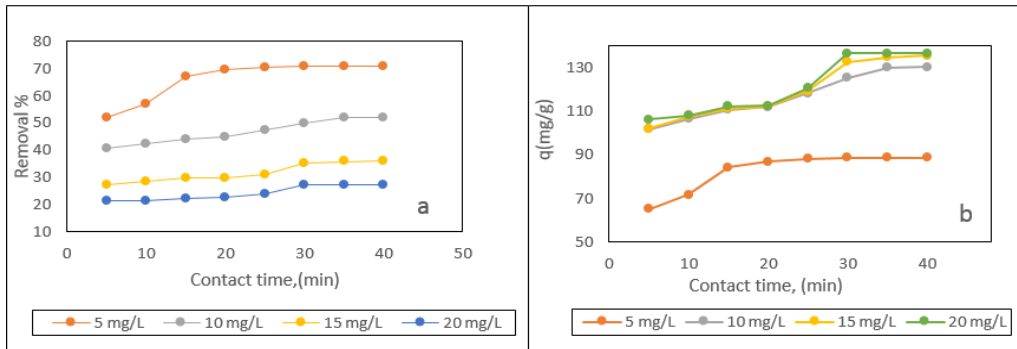
Figure. (6): (a) Removal efficiency of Pb +2 ions on graphene as a function of contact time (pH=4, dose =40 mg/L) (b) Adsorbed capacity (q mg/g) of Pb +2 ions on graphene as a function of contact time (pH=4, dose =40 mg/L)
