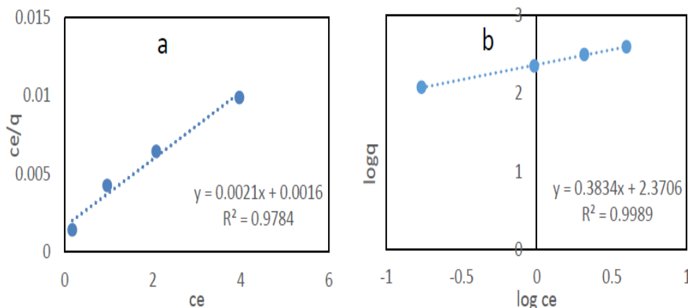
Figure (9): Isotherm model of Pb +2 ions adsorption onto graphene :( a) Langmuir (b) Freundlich (pH=6.2, dose =40 mg/L, contact time=35 min)
