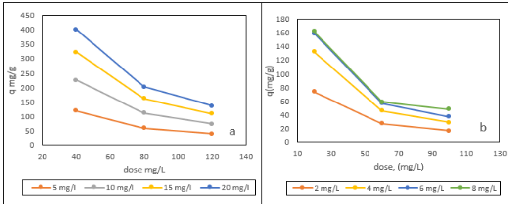
Figure (8): (a) Adsorbed capacity (q mg/g) of Pb 2+ ions on graphene as a function of dose (PH=6.2, contact time =35 min), (b) Adsorbed capacity (q mg/g) of Cd 2+ ions on graphene as a function of dose (PH=5.2, contact time =40 min)
