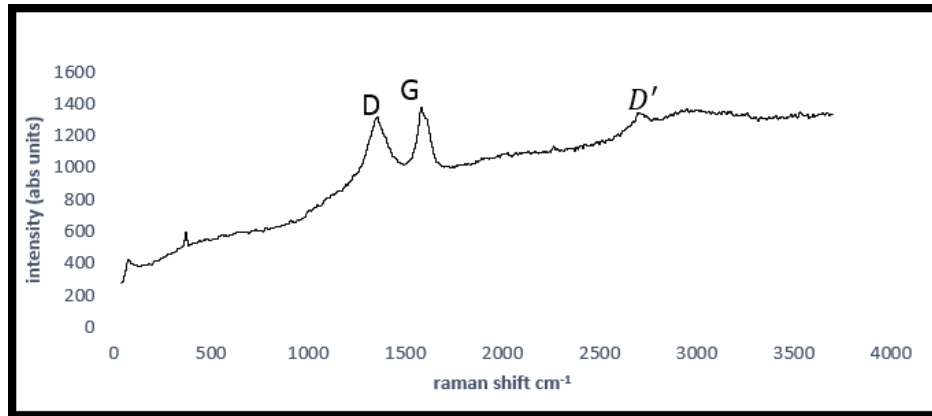
Figure (4): Raman spectrum of graphene from experiment (electrochemical exfoliation- graphite- graphite electrode)
