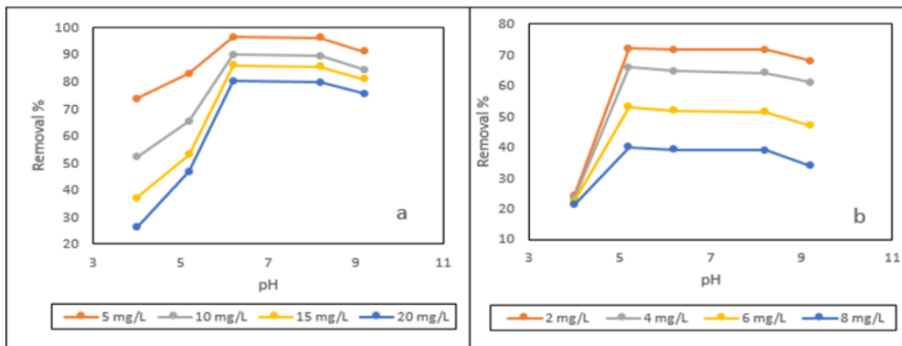
Figure (7): (a) Removal efficiency of Pb +2 ions on graphene as a function of pH (dose =40 mg/L, contact time =35 min), (b) Removal efficiency of Cd +2 ions on graphene as a function of pH (dose =20 mg/L, contact time =40 min)
