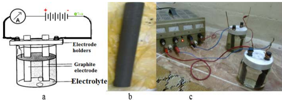
Figure.( 1): a/ schematics setup, b/ Graphite rod, c/ Experimental setup
