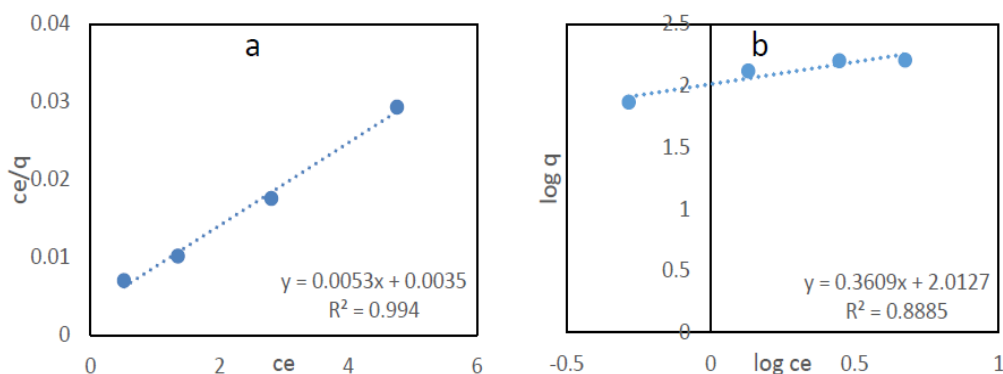
Figure (10): Isotherm model of Cd +2 ions adsorption onto graphene :( a) langmuir (b) Freundlich (pH=5.2, dose =20 mg/L, contact time=40 min)
